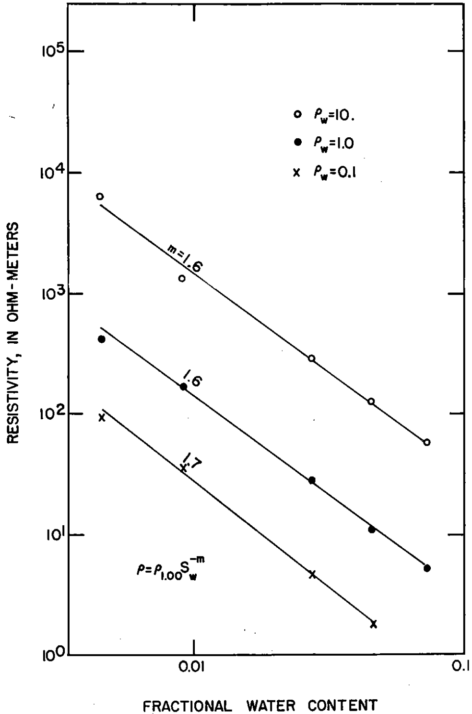
Figure 5.--Resistivity as a function of fractional water content for various water resistivities for sample A at a frequency of 100 MHz.
