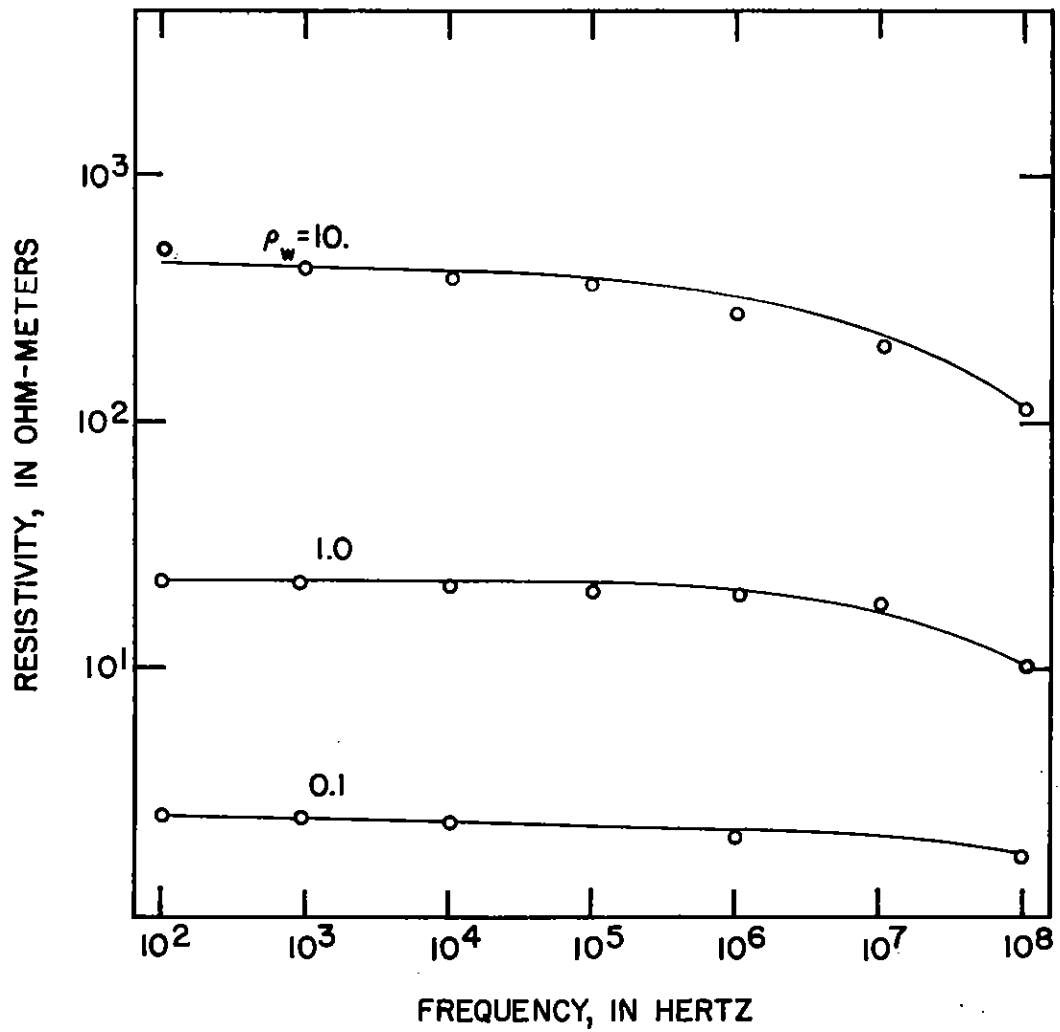
Figure 2.--Resistivity as a function of frequency for various water resistivities for sample A with a fractional water content of 0.47.
