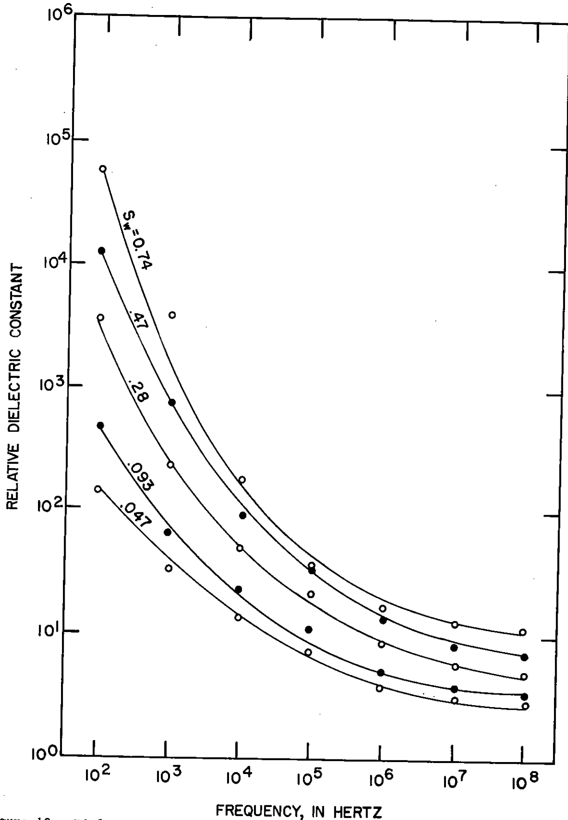
Figure 10.--Dielectric constant, as a function of frequency for various water contents for sample B containing 10.0 ohm-m water.
