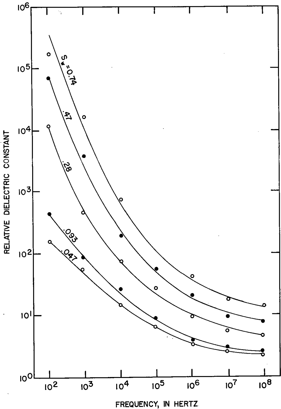
Figure 7.--Dielectric constant as a function of frequency for various water content for sample A containing 10 ohm-m water.
