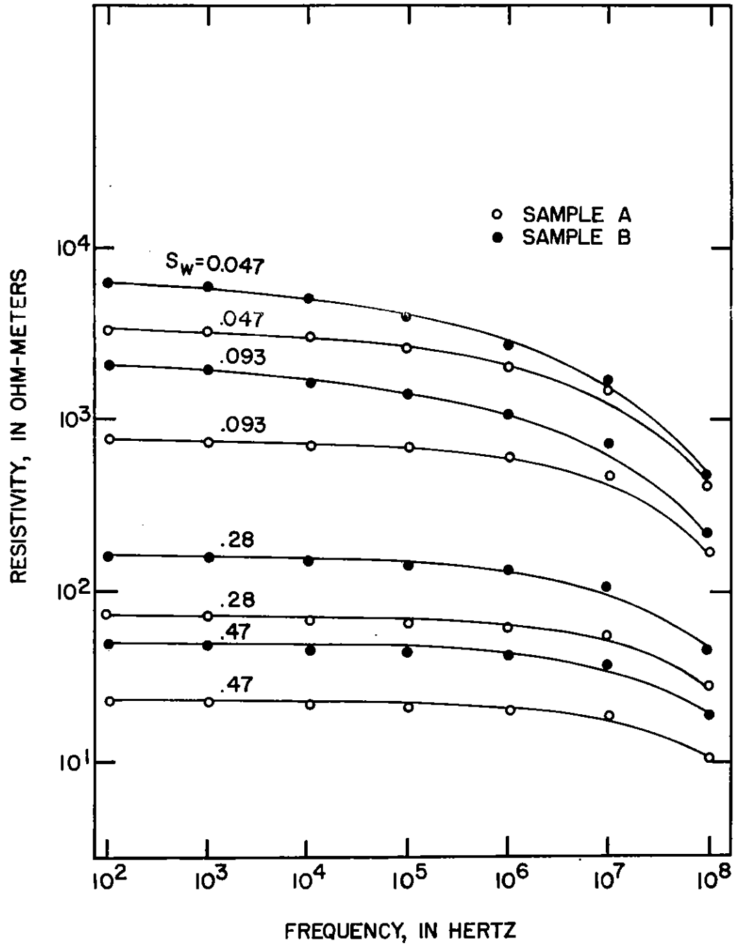
Figure 3.--Resistivity as a function of frequency for various water contents for samples A and B containing 1.0 ohm-m water.
