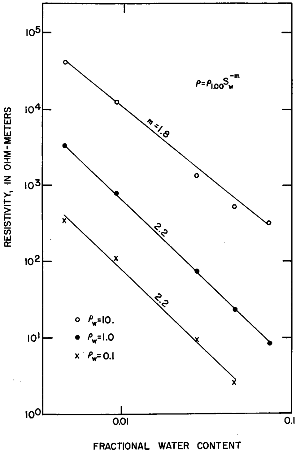
Figure 4.--Resistivity as a function of fractional water content for various water resistivities for sample A at a frequency of 100 Hz.
