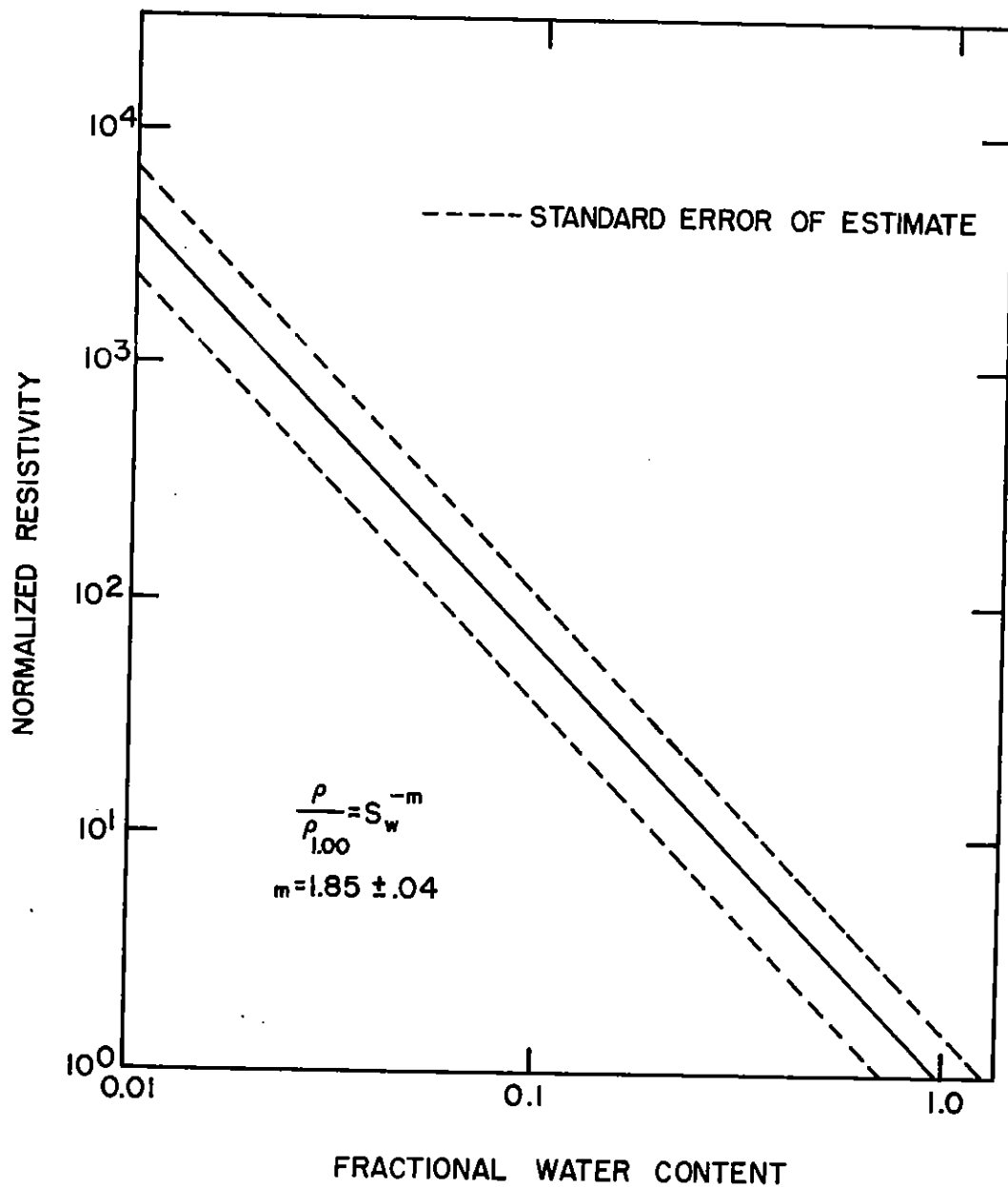
Figure 6.--Normalized resistivity as a function of water content.
