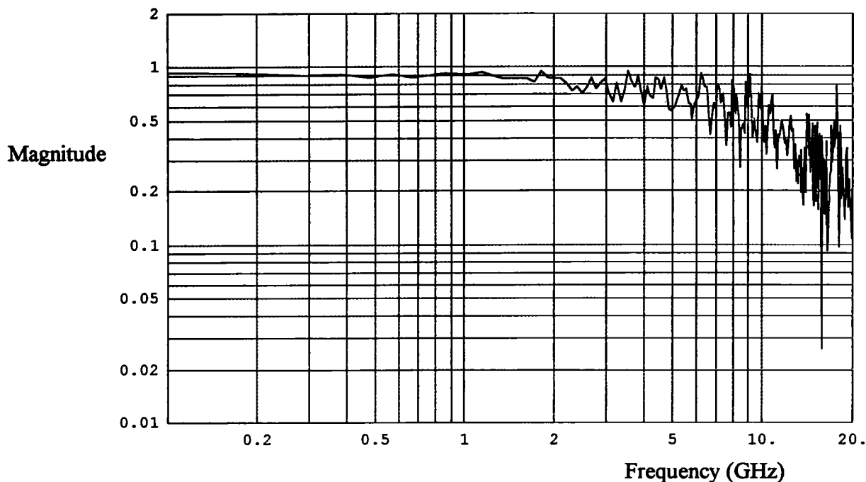
Figure 7.7. Ratio of the derivative of the reflection from the short to the derivative of the source. The data is probably valid only up to 10 GHz.
