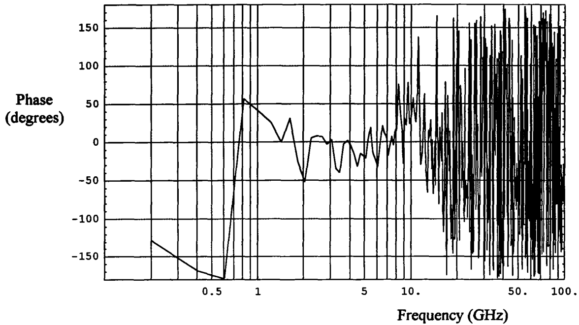
Figure 8.14. The phase of h^2(\omega)/f_g after unwrapping, just before taking the complex square root.
