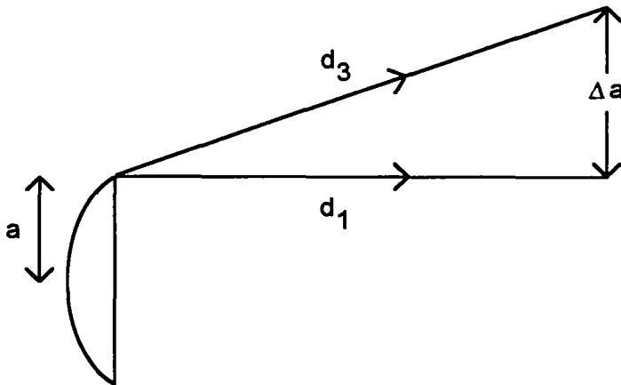
Figure 4.2. Calculation for determining the size of the reflecting plate.
