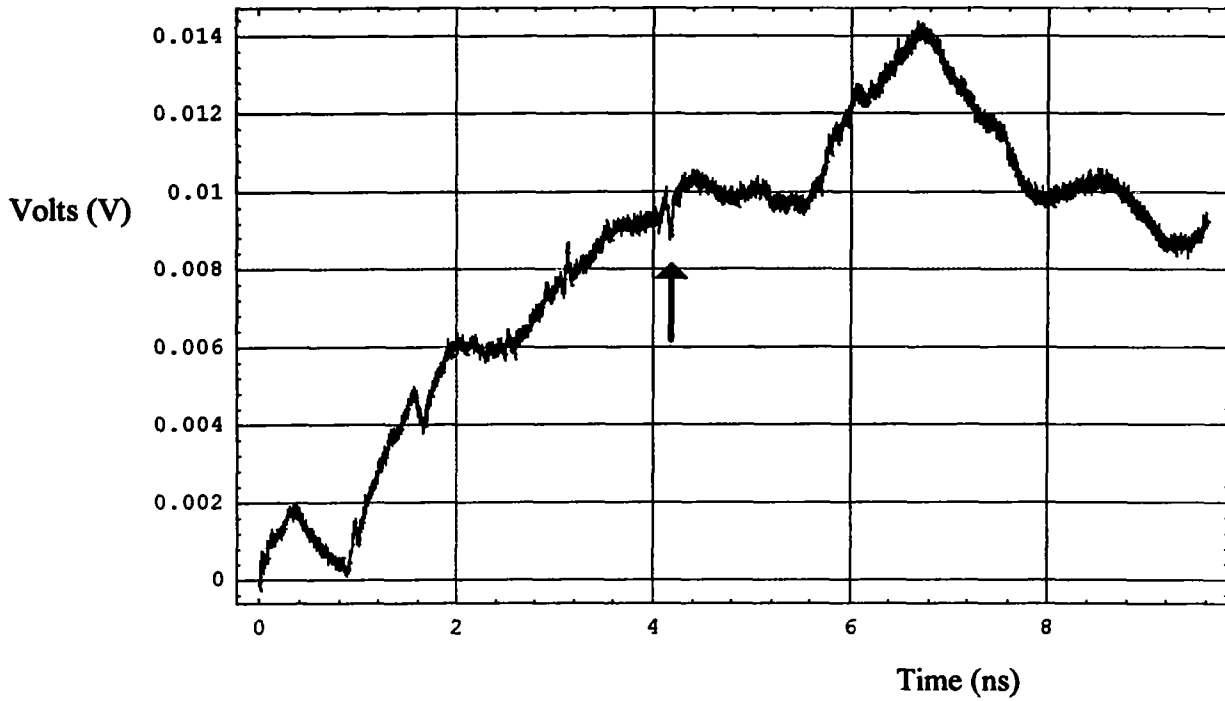
Figure 8.2. The background (no reflector plate).
