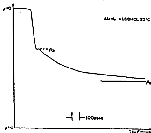
Figure 10.3. Sample TDR (reflection coefficient vs. time) for a reflection from Amyl Alcohol; from [11].
