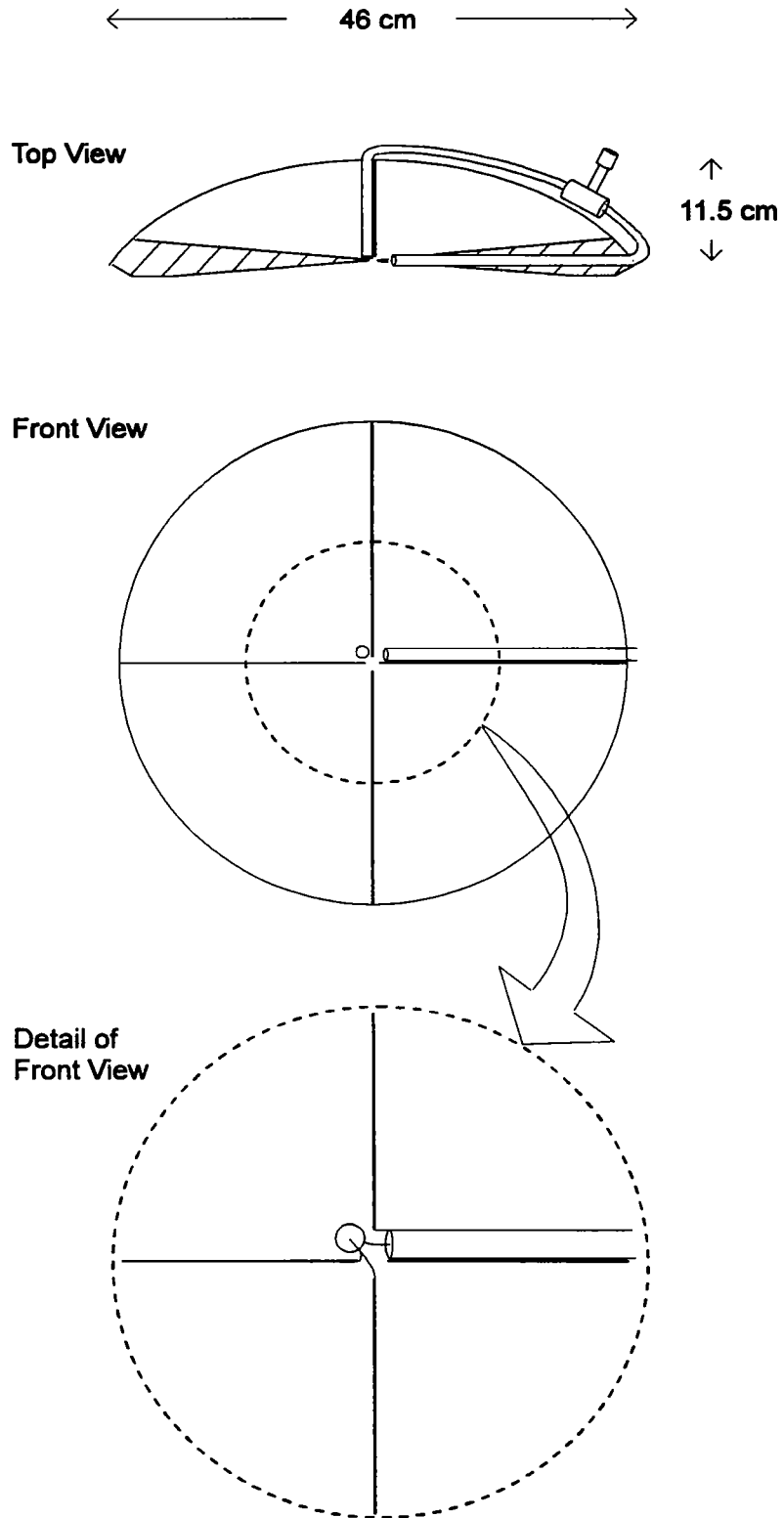
Figure 7.1. The reflector IRA as built.
