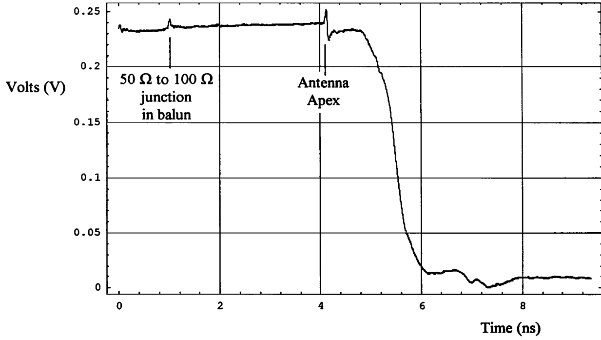
Figure 7.9. The reflection from the antenna.
