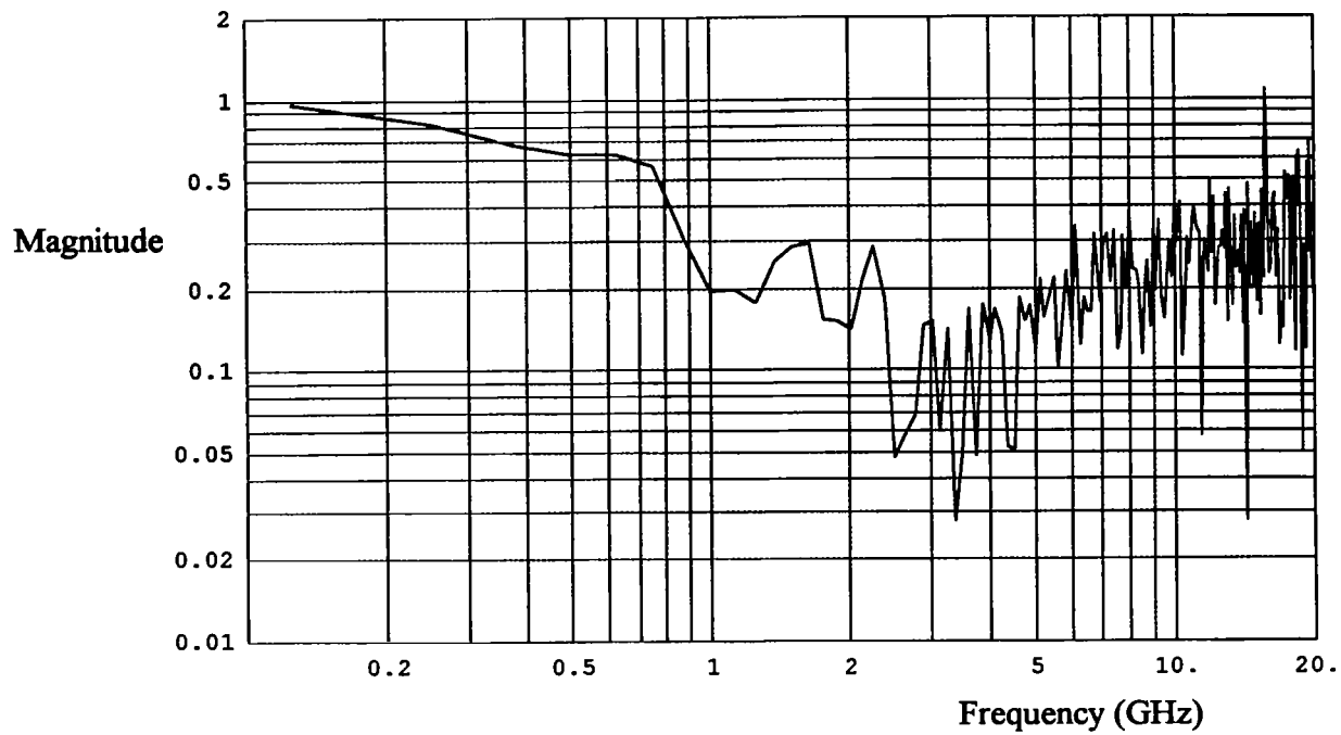
Figure 7.12. Return loss of the IRA, calculated as the frequency domain ratio of the derivative of the reflection from the antenna to the derivative of the input source voltage.
