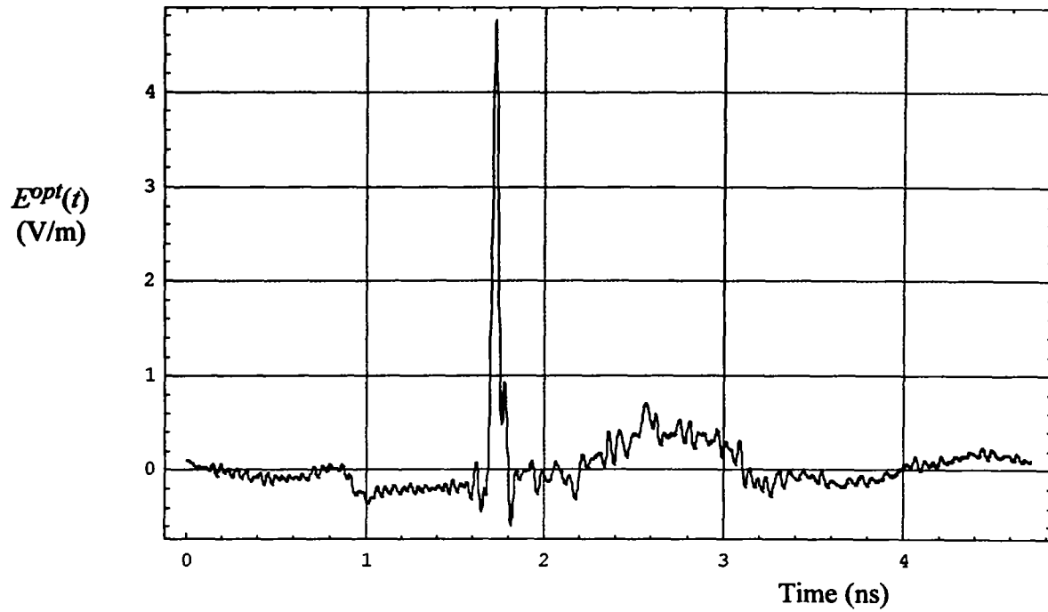
Figure 9.10. A rescaling of Figure 9.8 to allow one to predict the field radiated by the antenna scaled to a 1 meter distance, when excited by a 1 V step pulse with infinitely fast risetime.
