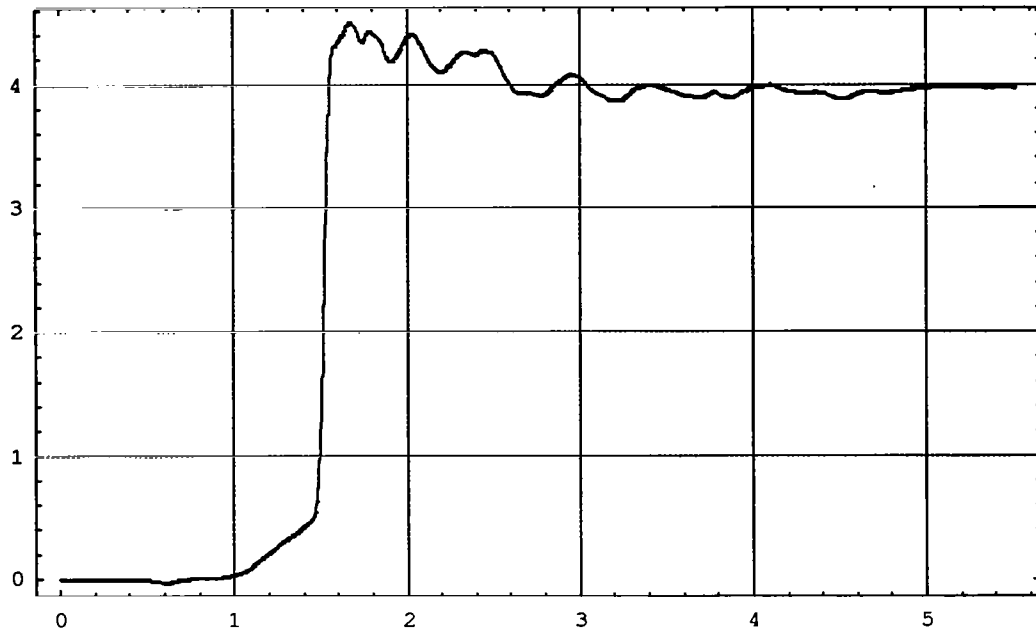
Figure 9.6. The source voltage sampled at 0.46 ps/sample.
