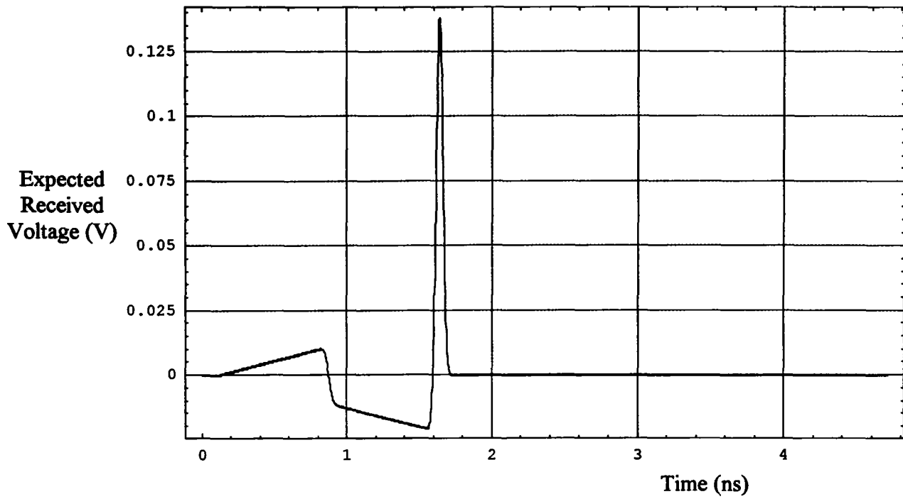
Figure 9.4. Expected received voltage.
