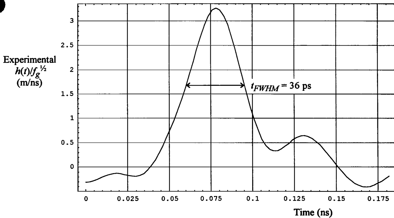
Figure 9.9. Close-up of the peak of Figure 9.8.
