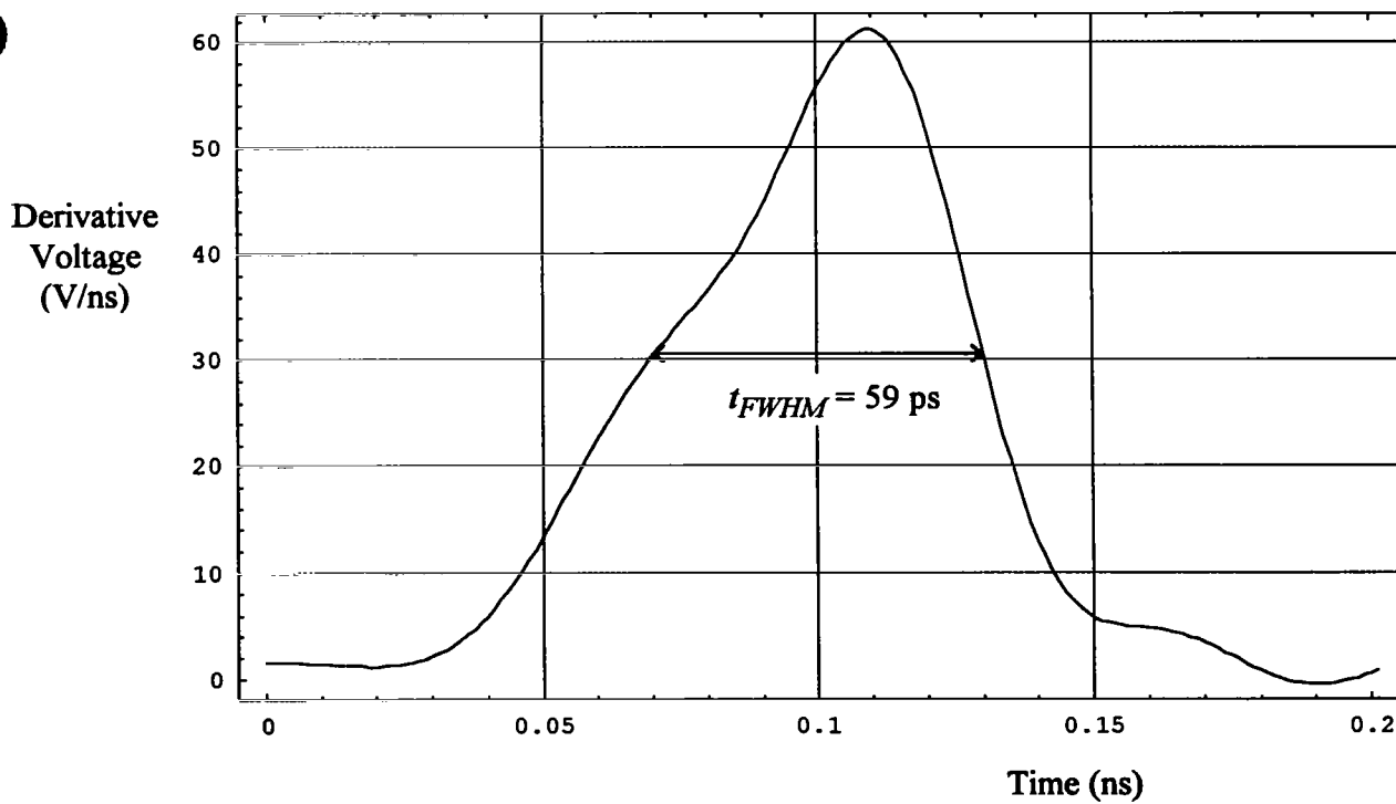
Figure 9.3. The derivative of the source voltage, after filtering and taking the derivative.
