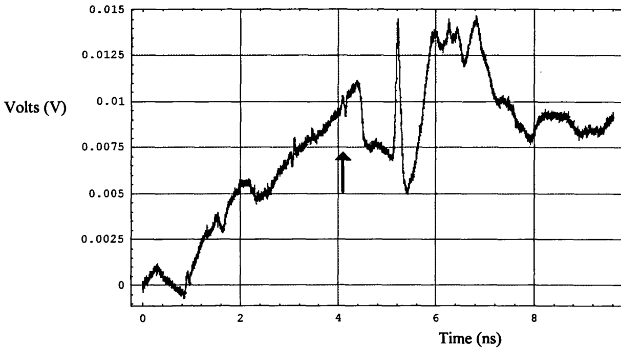
Figure 8.3. The raw received voltage (with the reflector plate in place), in the presence of a background.
