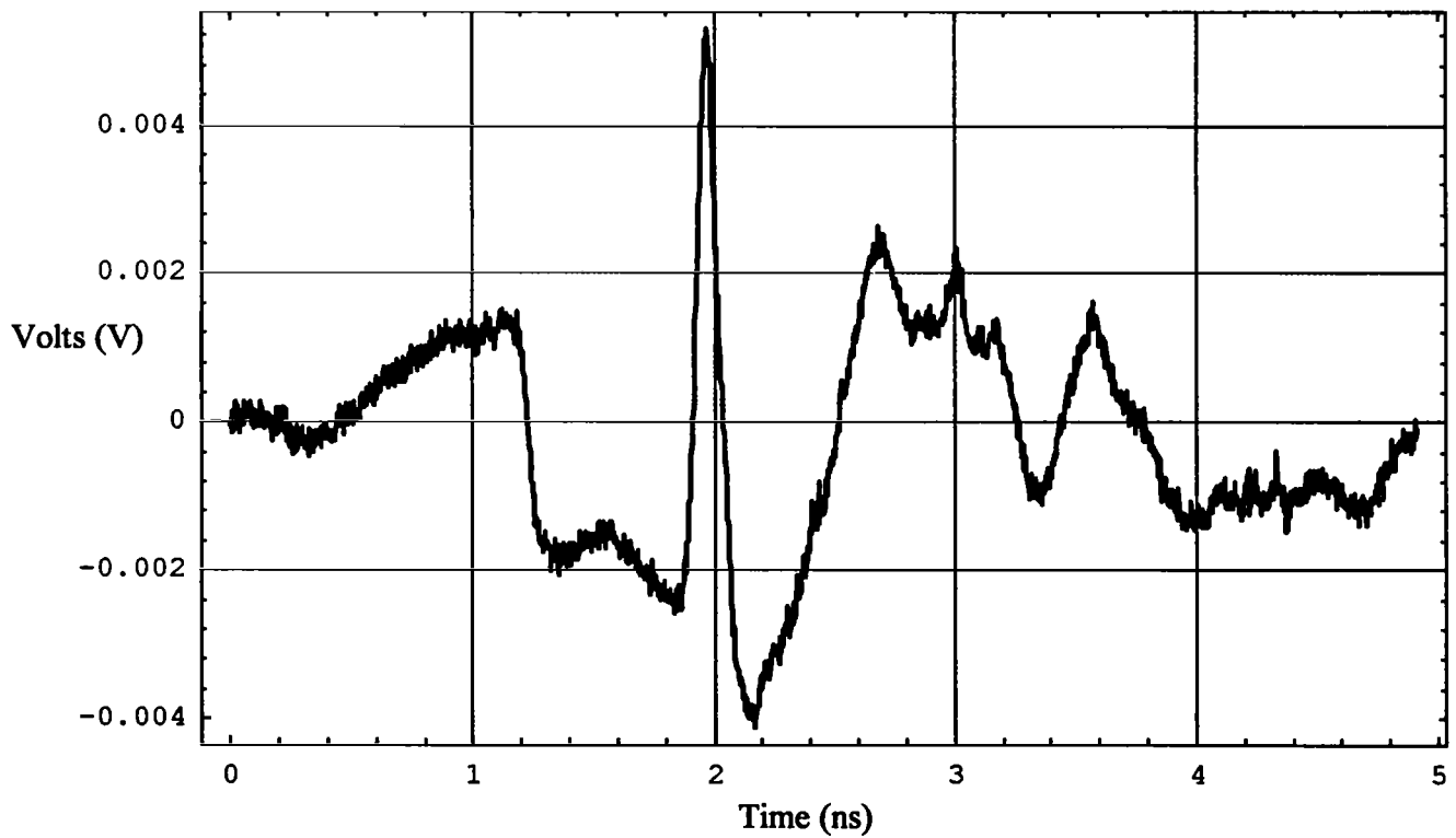
Figure 8.5. The received voltage after a 3:1 data averaging and truncation at early and late times.
