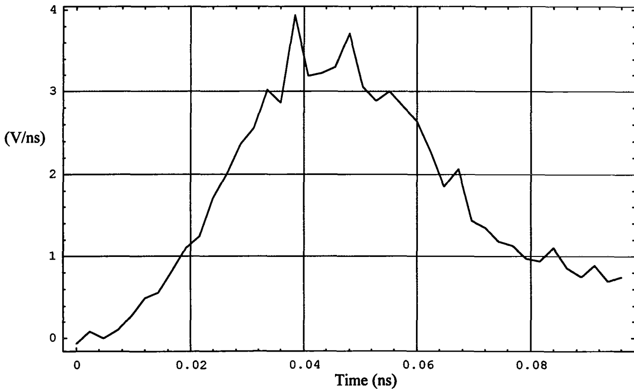
Figure 8.11. A close-up of the derivative of the voltage reflected from the short.
