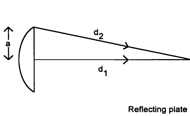
Figure 4.1. Far field calculation.
