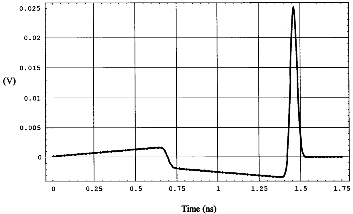
Figure 8.13. The predicted received voltage. (Compare to Figure 8.7.)
