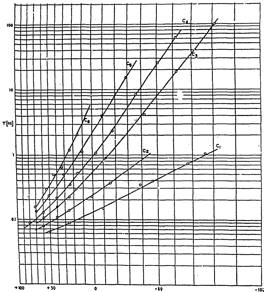
Figure 10.4. Relaxation time as a function of temperature (degrees C) for various alkyl alcohols, from [11].
