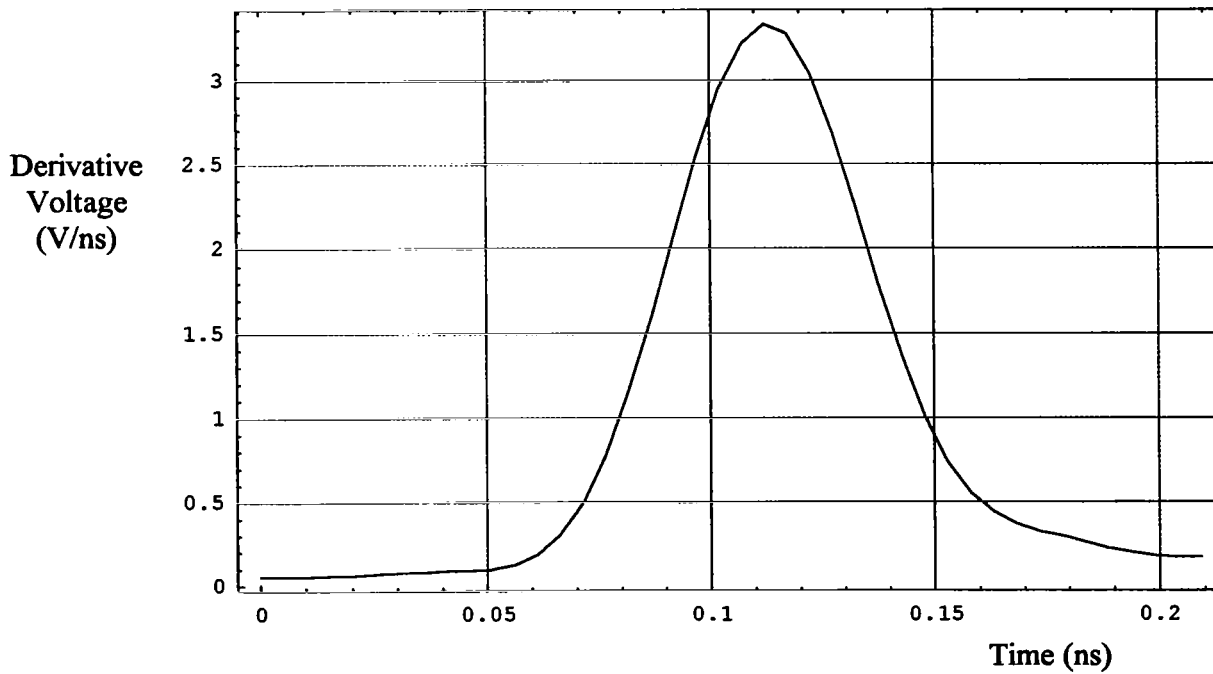
Figure 7.6. Derivative of the reflection from the shorted apex. Note that t_{FWHM} = 51.7 ps, area = 0.197 V, and the peak = 3.34 V/ns.
