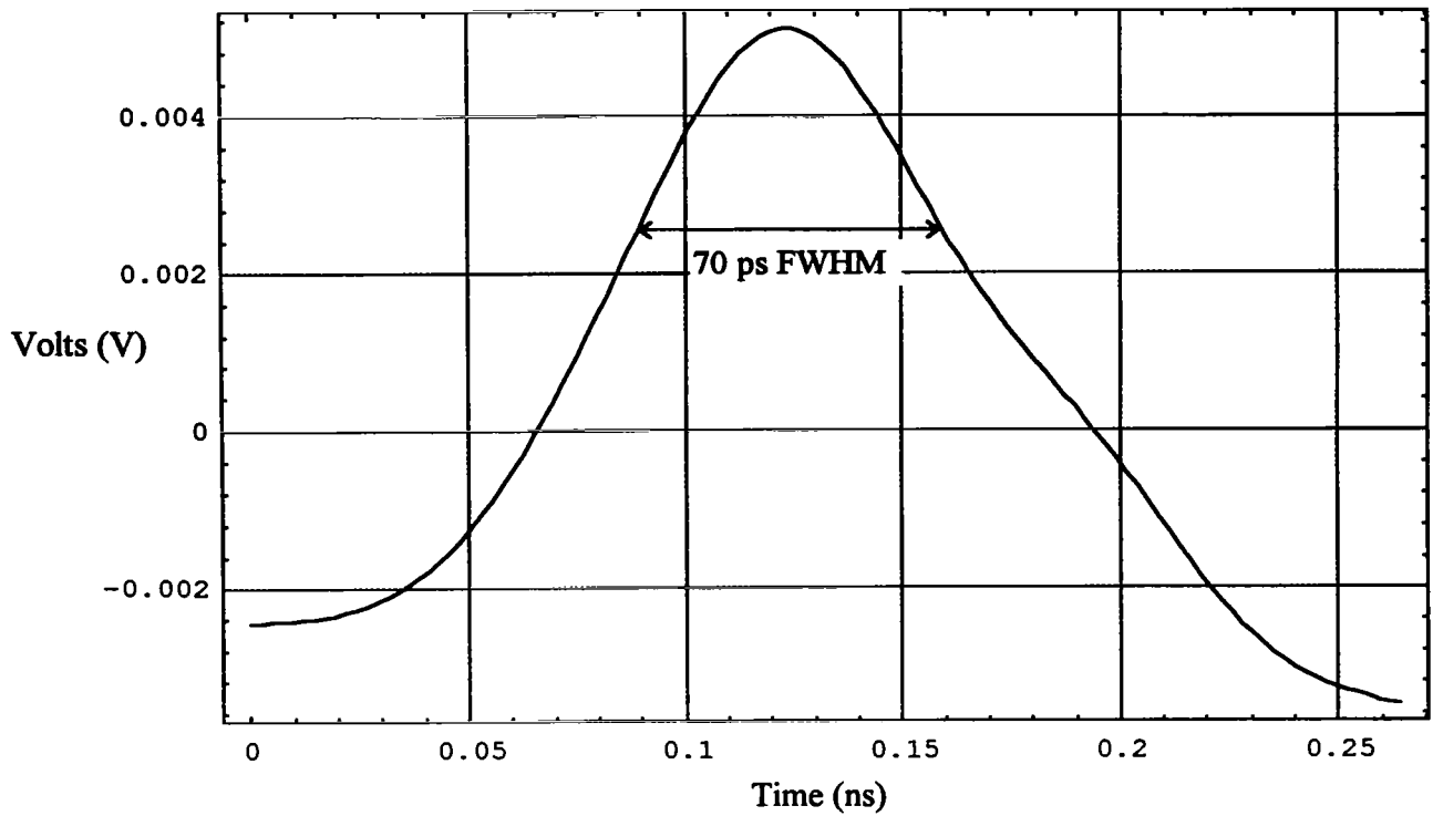
Figure 8.8. A close-up of the impulse portion of Figure 8.7.
