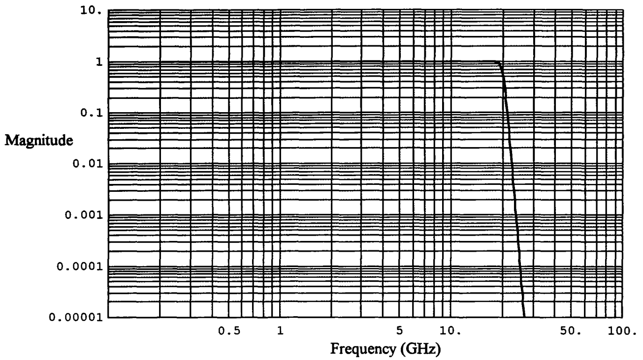
Figure 8.6. The 20 th -order modified Butterworth filter used on the data
