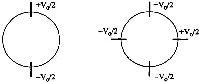
Figure 2.2. Reflector IRA configurations with two and four arms.
