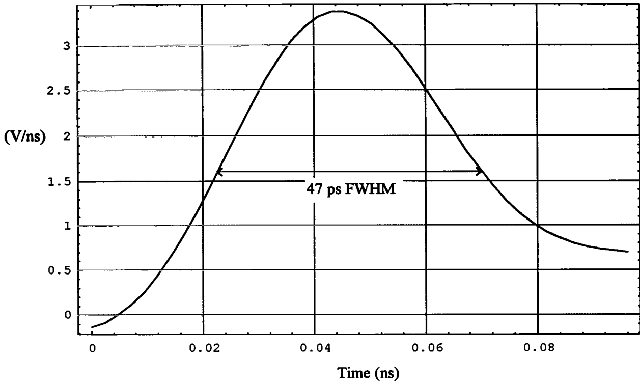
Figure 8.12. The derivative of the voltage reflected from the short after filtering.
