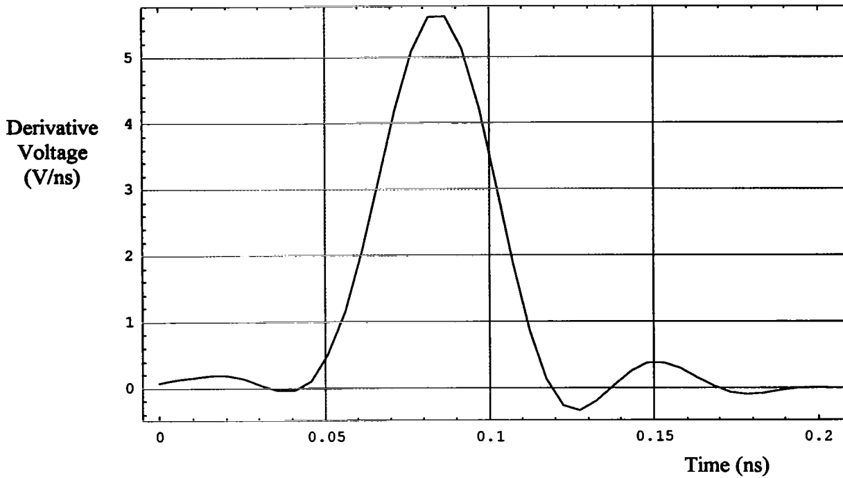
Figure 7.5. Derivative of the source waveform. Note that t_{FWHM} = 38.5 ps, area = 0.225 V, and the peak = 5.61 V/ns.
