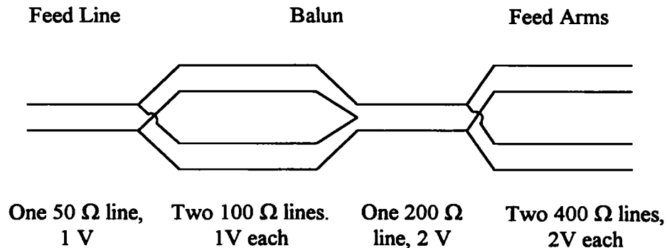
Figure 5.2. The voltages and feed impedances of the geometry at various points along the feed.
