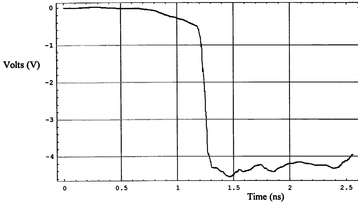
Figure 9.2. The source voltage, taken at a sweep speed of 0.25 ps/sample.
