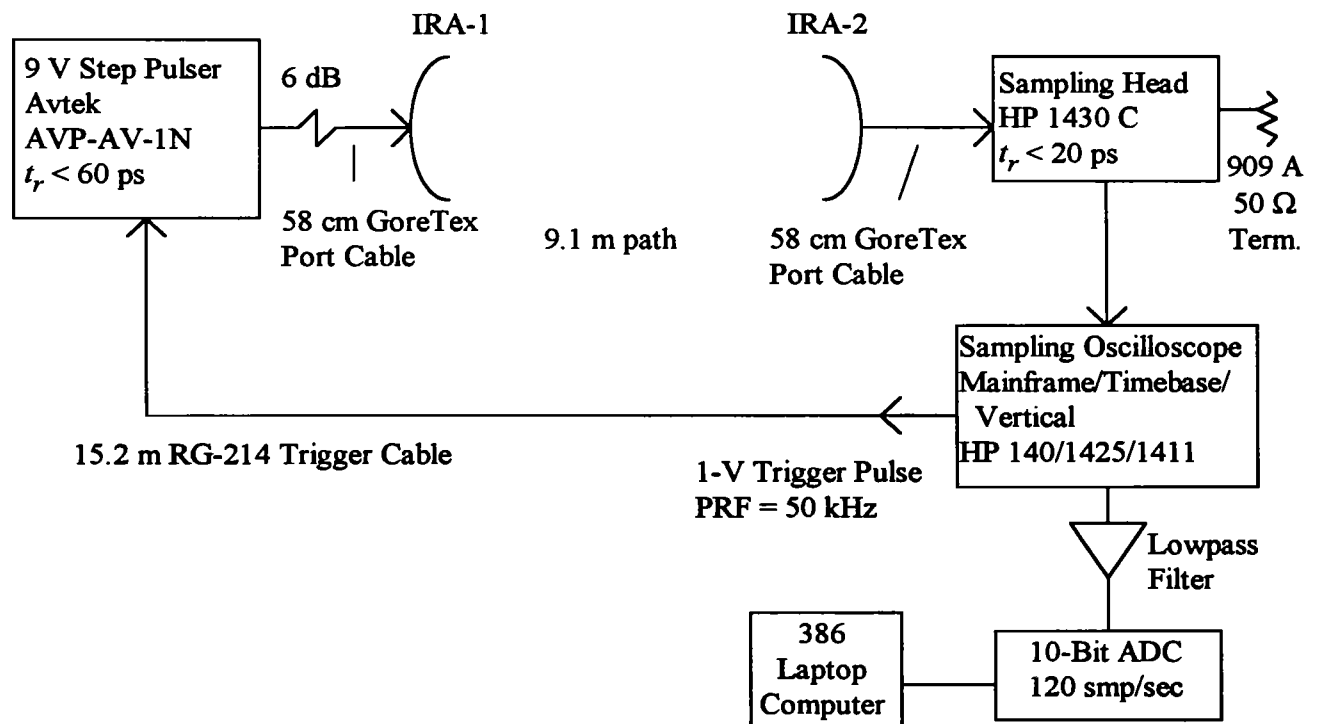
Figure 9.1. Outdoor Antenna Measurement Setup
