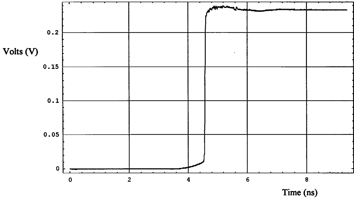
Figure 7.8. The source waveform.
