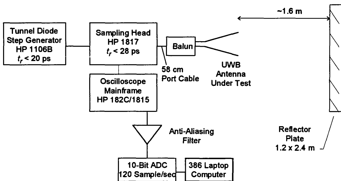
Figure 8.1. The experimental configuration used to measure the IRA's radiated field, using a single antenna with a large reflecting plate.
