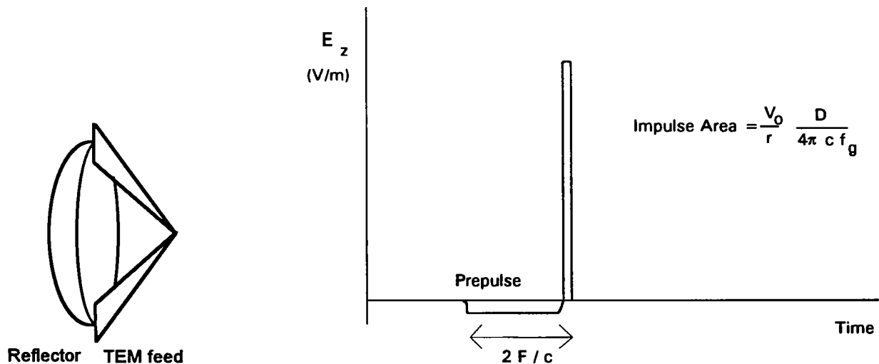
Figure 2.1. An example of a reflector IRA (left) and the radiated electric field on boresite when the antenna is driven by a fast, smooth step-function voltage (right).
