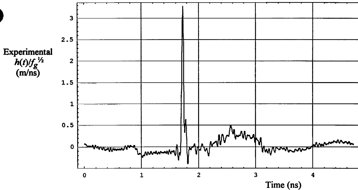
Figure 9.8. Processed h(t)/f_g^{1/2} .
