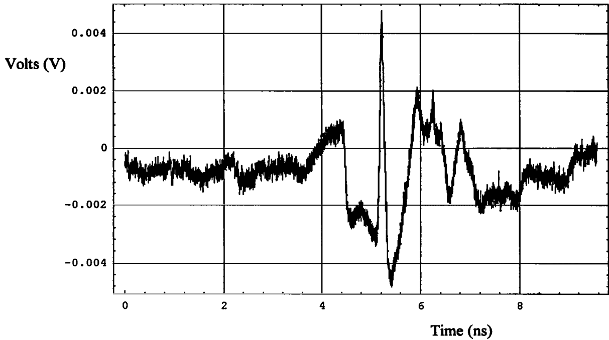
Figure 8.4. The received voltage after subtracting out the background. Note that the bump near 4.2 ns has been removed.
