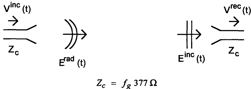
Figure 3.1. The relevant quantities for specifying antenna performance in the time domain for transmission (left) and reception (right).
