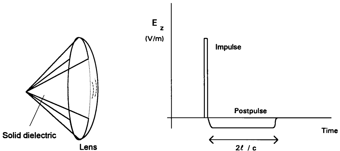
Figure 2.5. A solid dielectric lens IRA (left) and an example of its output (right).
