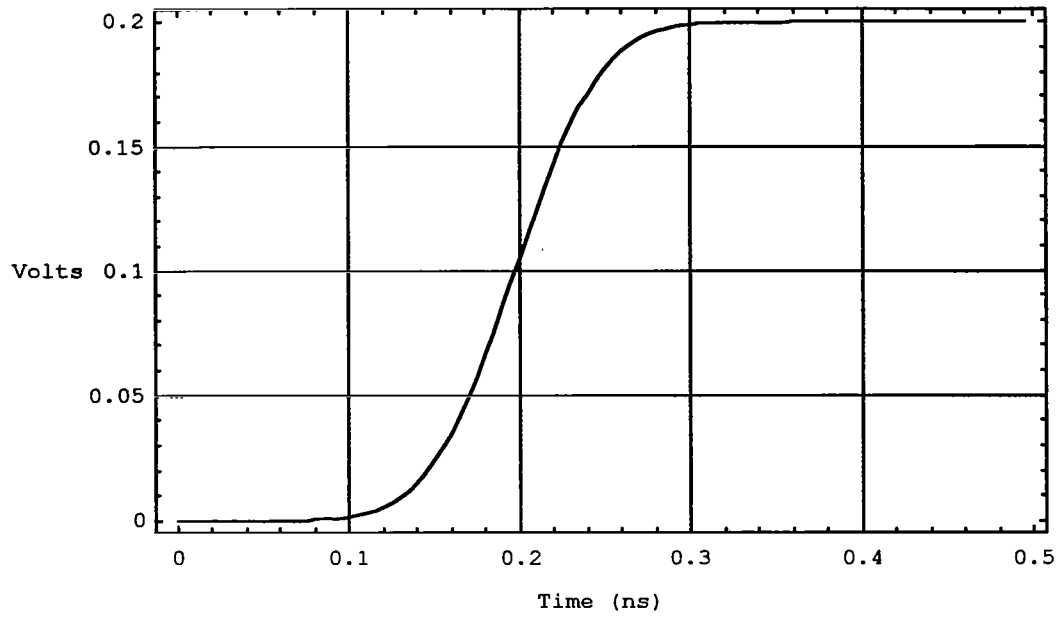
Figure 6.2. Driving voltage scaled to the parameters of the current problem.
