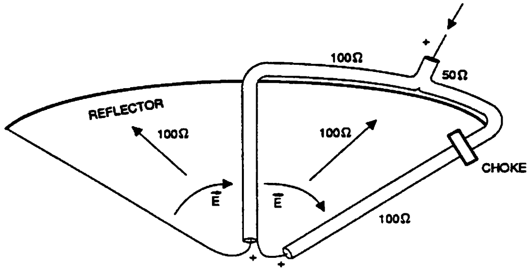
Figure 5.1. A 50 \Omega to 200 \Omega balun for a reflector IRA.
