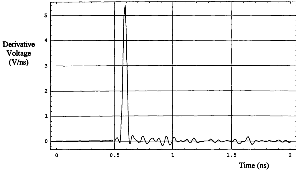
Figure 7.10. Derivative of the input voltage. Note that t_{FWHM} = 39.2 ps, area = 0.222 V, and the peak = 5.40 V/ns.
