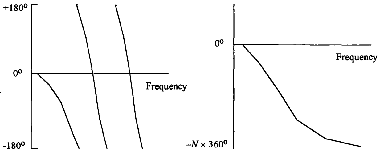
Figure 3.2. Illustration of phase unwrap before (left) and after (right).
