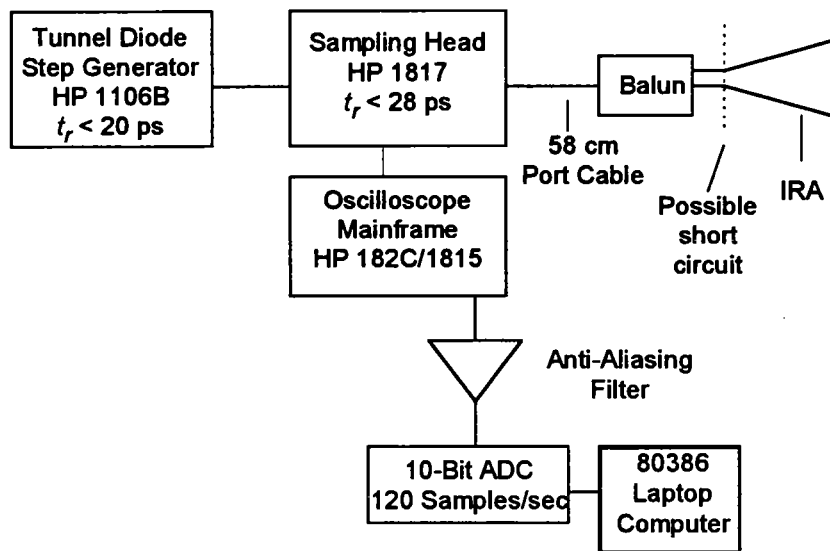
Figure 7.2. The experimental configuration used to test the frequency response of the balun and also used to measure the TDR of the IRA radiating into free space.
