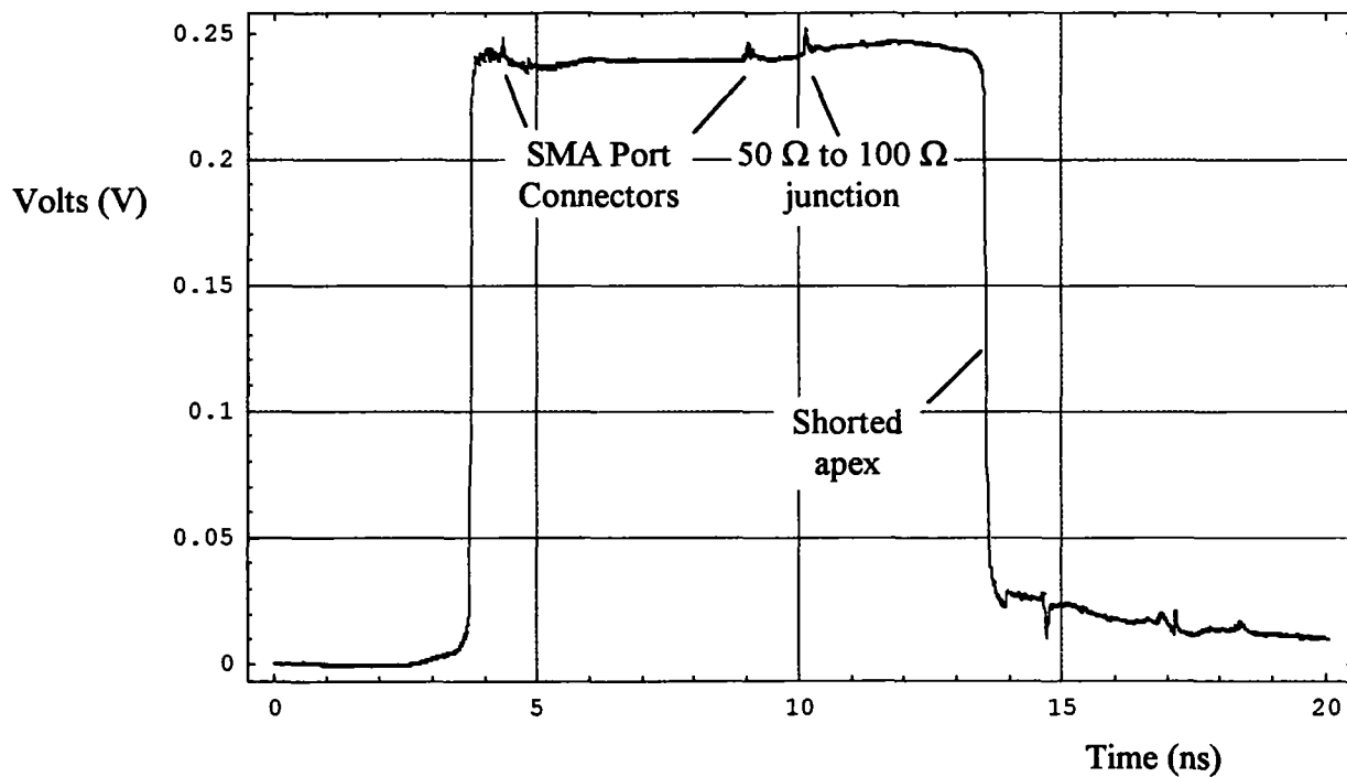
Figure 7.4. The reflection from the short.
