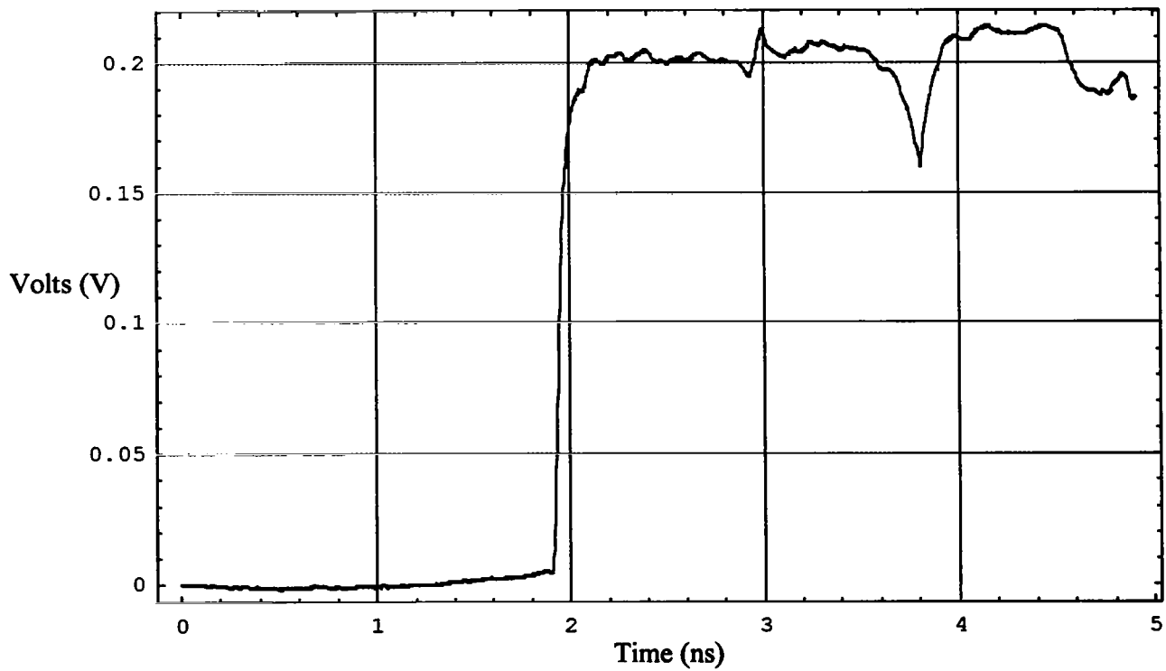
Figure 8.9. The voltage reflected from the shorted apex.
