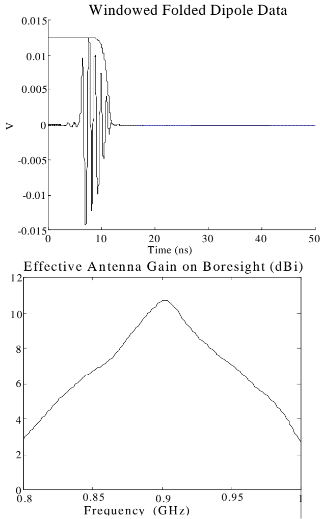
Figure 7.2. Gain of M^2 folded dipole from truncated time domain data.
