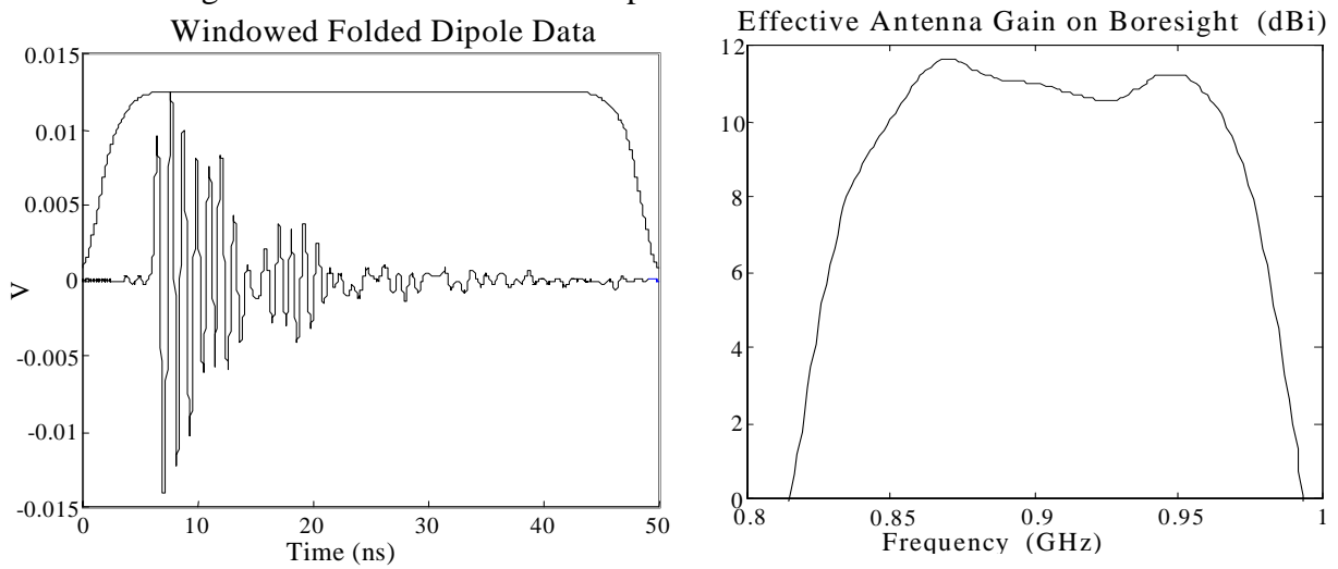
Figure 7.2. Gain of M^2 folded dipole from truncated time domain data.
