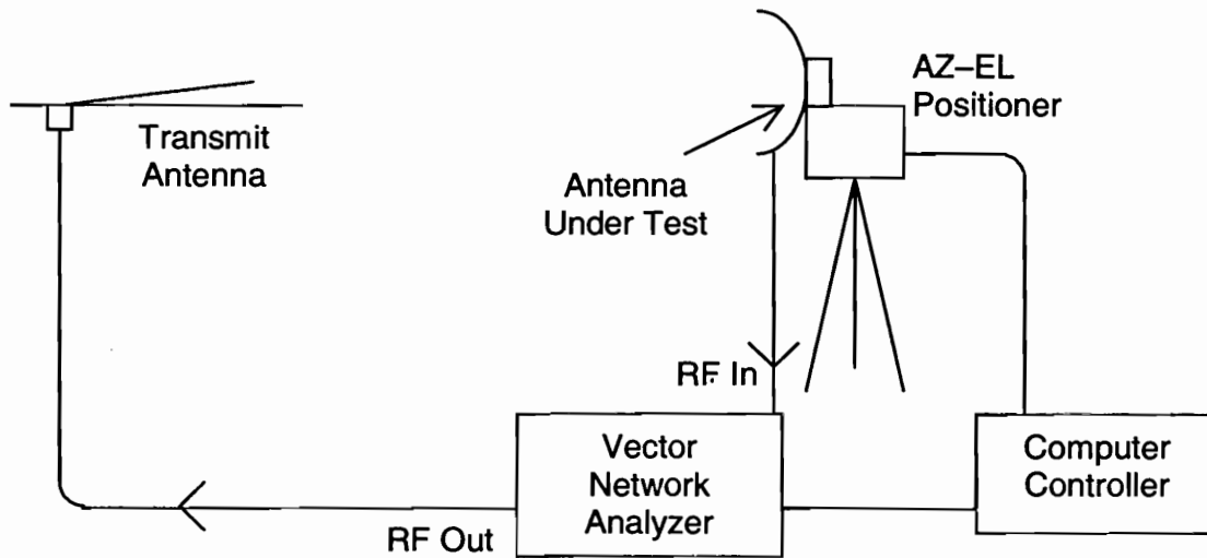
Figure 1. Frequency domain antenna measurement system.
