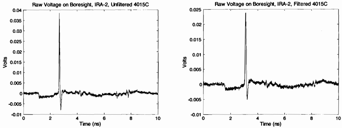
Figure 13. Raw response of the IRA-2 for unfiltered and risetime-filtered PSPL 4015C. The unfiltered peak response is 38 mv, with a FWHM of 51 ps. With the 70 ps gaussian risetime filter, the peak response is 24 mv, with a FWHM of 75 ps.
