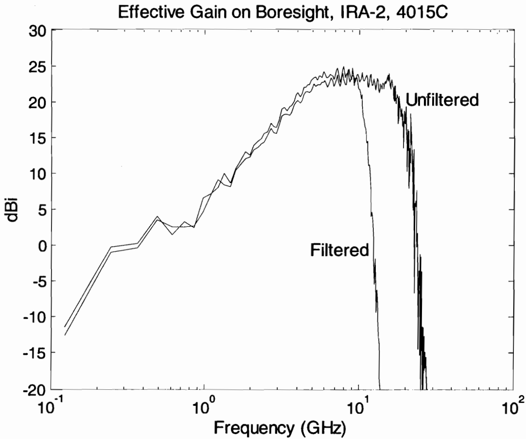
Figure 14. IRA-2 gain comparison, risetime-filtered and unfiltered source (semi-log plot).
