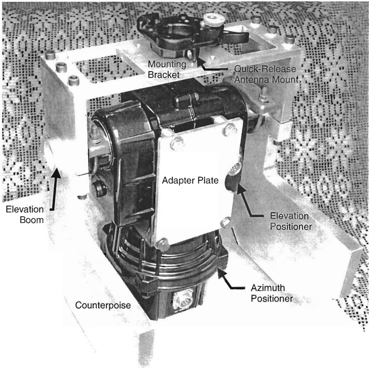
Figure 5. AZ-EL positioners with antenna mounting bracket and counterpoise.
