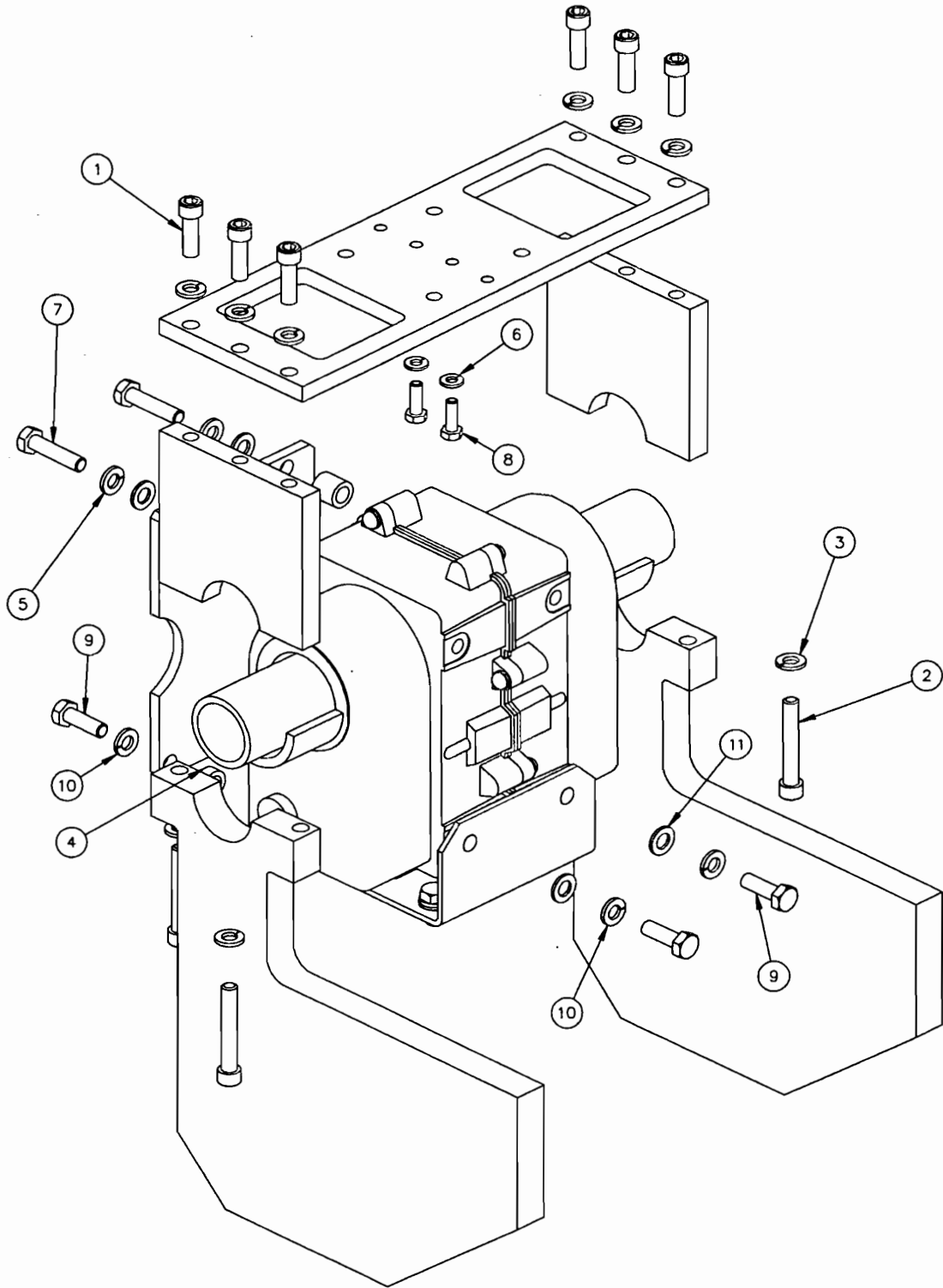
Figure 6. Assembly drawing for antenna mounting bracket and counterpoise with elevation positioner. In use, the bracket at the base of the elevation positioner is bolted to the top of the azimuth positioner.
