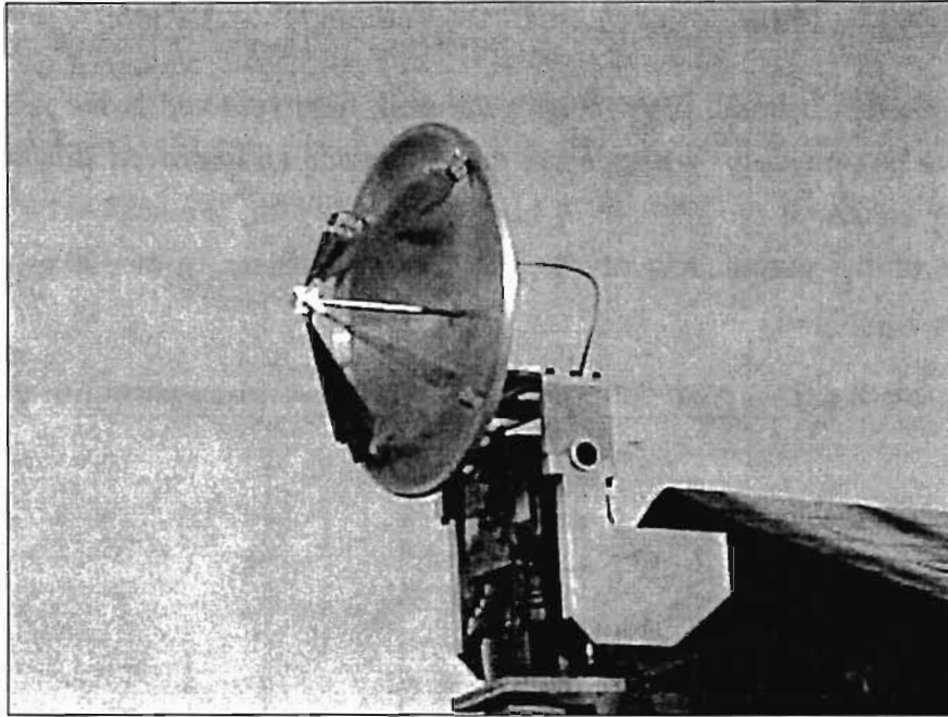
Figure 10. Antenna under test at time domain range. The antenna and AZ-EL positioner assembly is mounted on a raised platform affixed to the front wall of the instrumentation shed.
