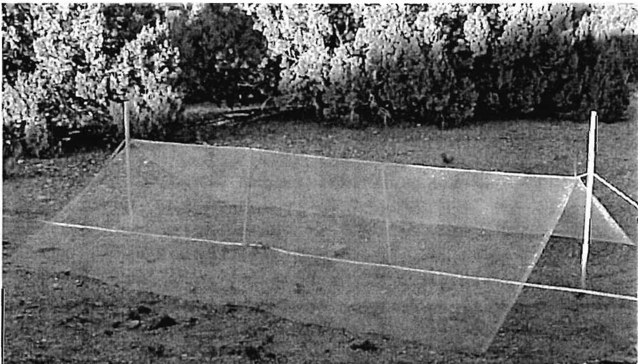
Figure 17. Tent-shaped reflector for mitigation of ground bounce. The ridge line of the metal mesh is parallel to the boresight direction.
