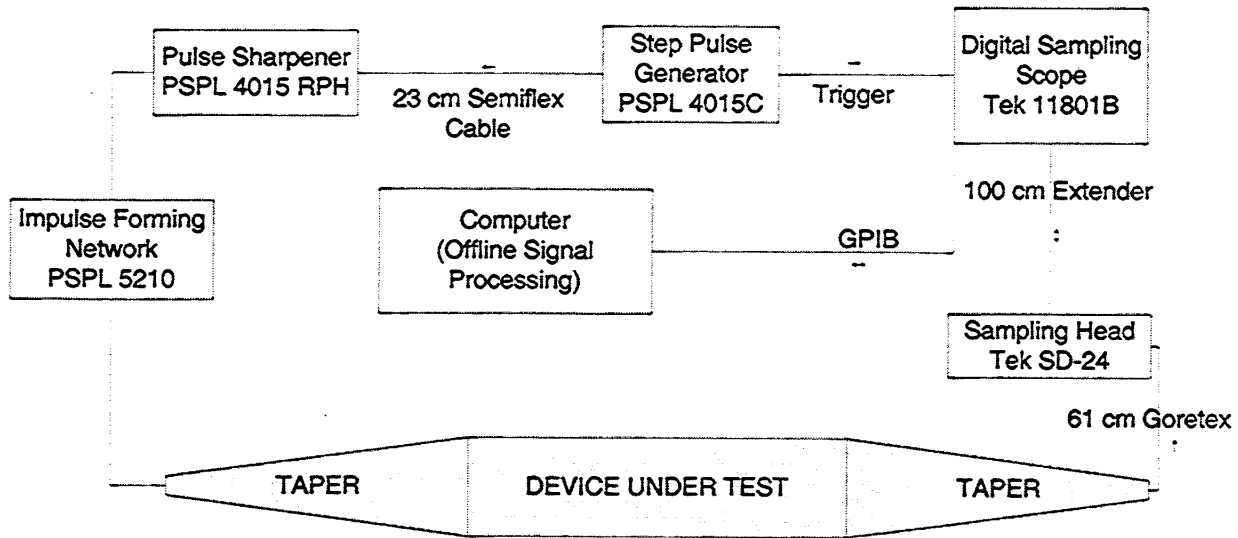
Figure 10. Equipment setup for coaxial transmission line measurements. The device under test (DUT) was either a 5.08 cm (2") square 90° coaxial bend or straight section loaded with a dielectric medium. Measurement waveforms were downloaded through the GPIB bus to a computer for offline signal processing.
