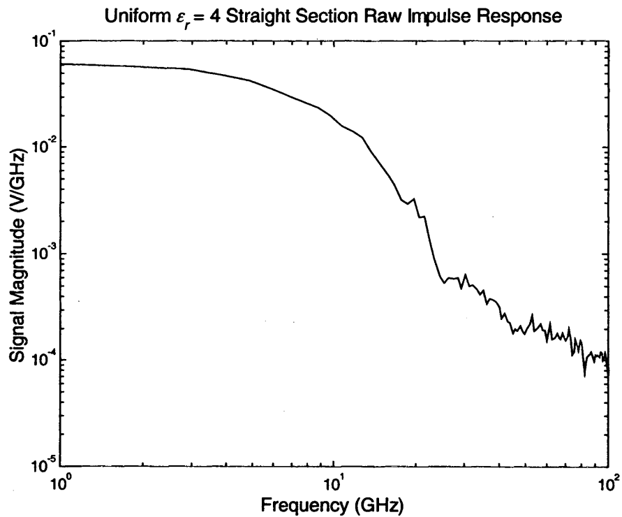
Figure 15. Raw impulse response for the 19.08 cm (7.51") straight section filled with a uniform \epsilon_r = 4 dielectric. The FWHM of the time-domain peak is 55 ps.
