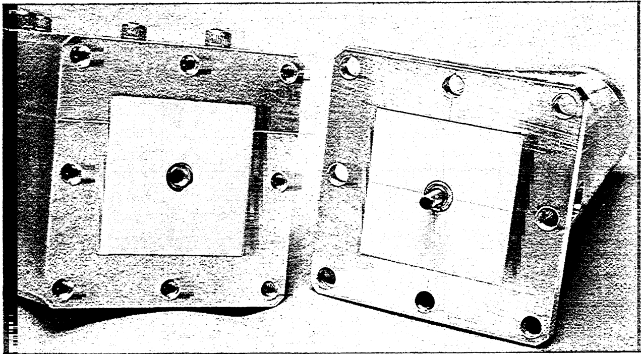
Figure 18. Layered dielectric bend (left), shown with one of two mating taper sections (right).
