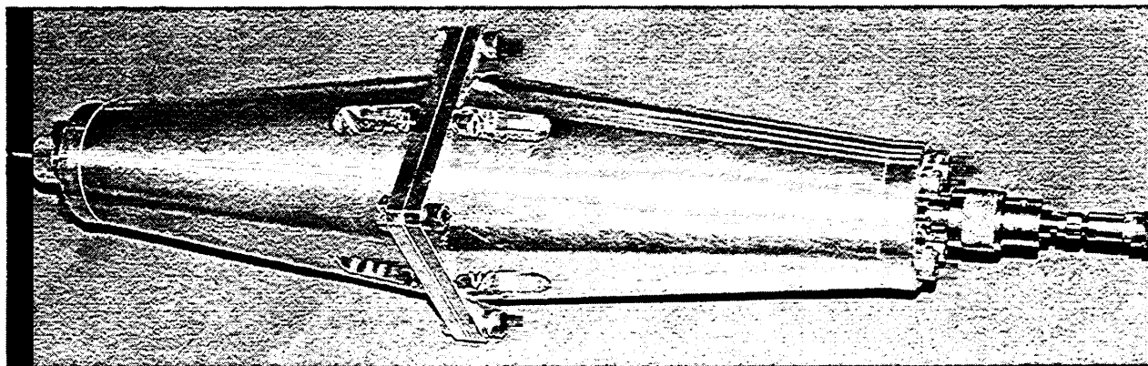
Figure 11. Tapered coaxial transmission line transition sections configured for a system response correction measurement.
