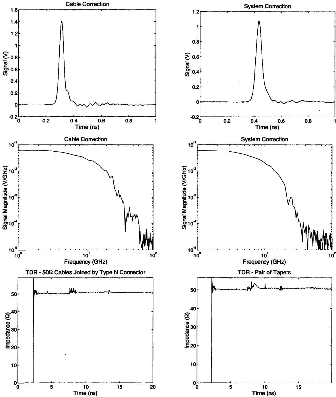
Figure 12. Cable and system impulse responses and TDR measurements. Plots of cable measurements are in the left column. System measurements are on the right.
