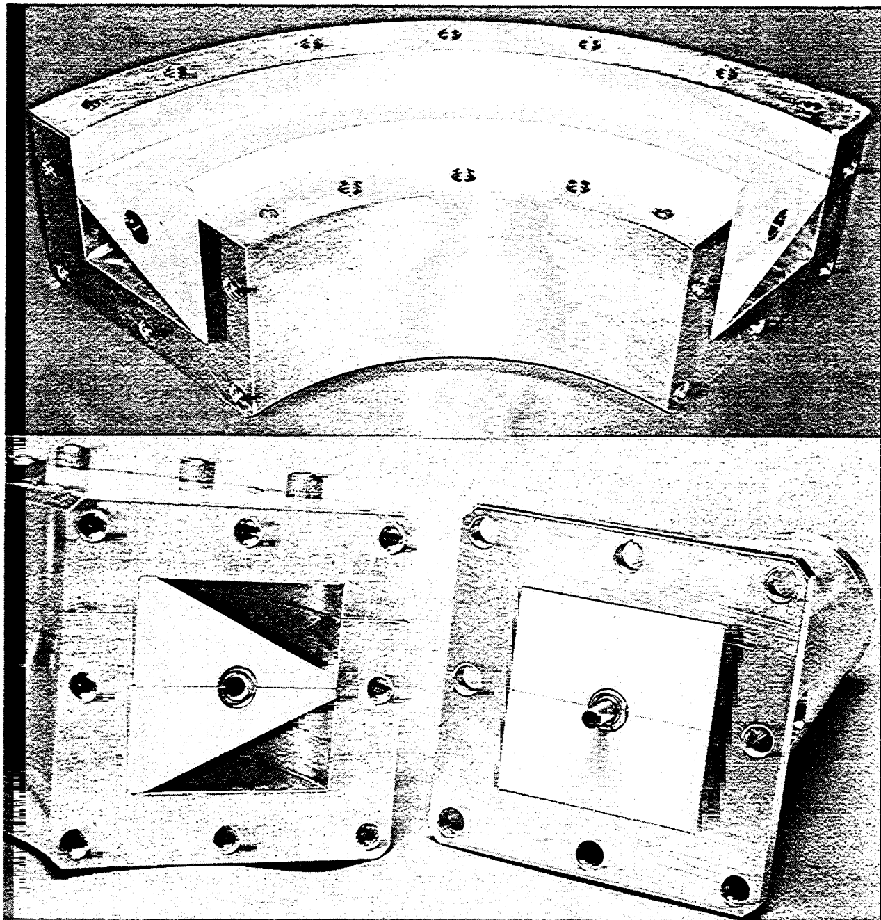
Figure 9. Sharp wedge partial dielectric fill design. The upper photograph shows the partially assembled bend. The lower shows an end view of the wedge-bend assembly, along with one of the two mating taper sections. The dielectric constant of the wedge material is 6.0; that of the taper material is 4.0.
