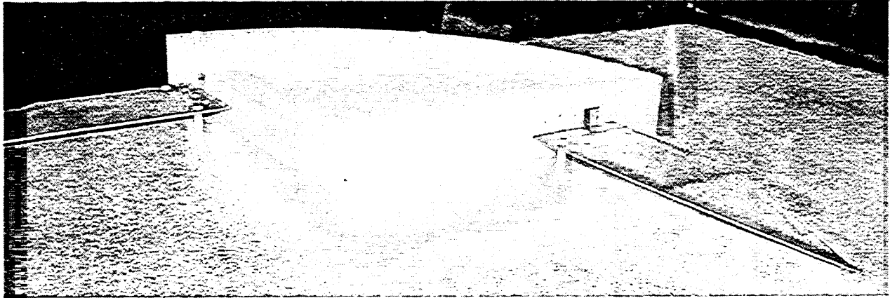
Figure 1. Strip transmission line bend approximately compensated by five uniform dielectric layers. Dielectric constants vary from 2.3 to 4.4. The strip width is 6.35 cm (2.5"), and has an inner radius of curvature of 12.95 cm (5.1").
