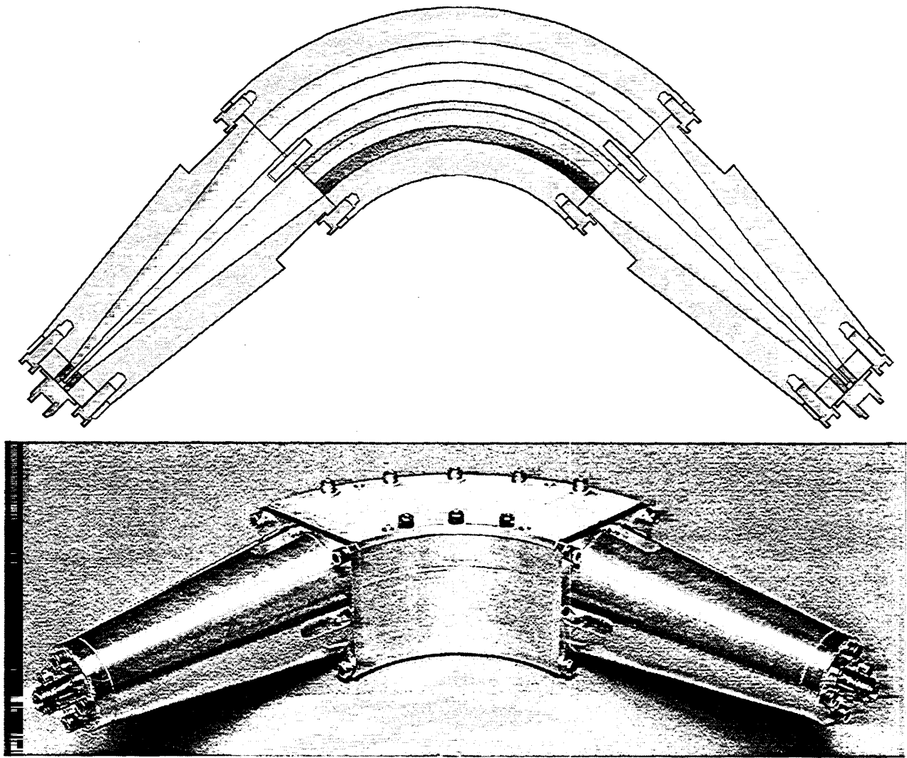
Figure 6. Square coaxial transmission line test fixture with 90° bend. The CAD drawing is a z-plane cut through the test fixture centerline. The photo is of the fully assembled test fixture.
