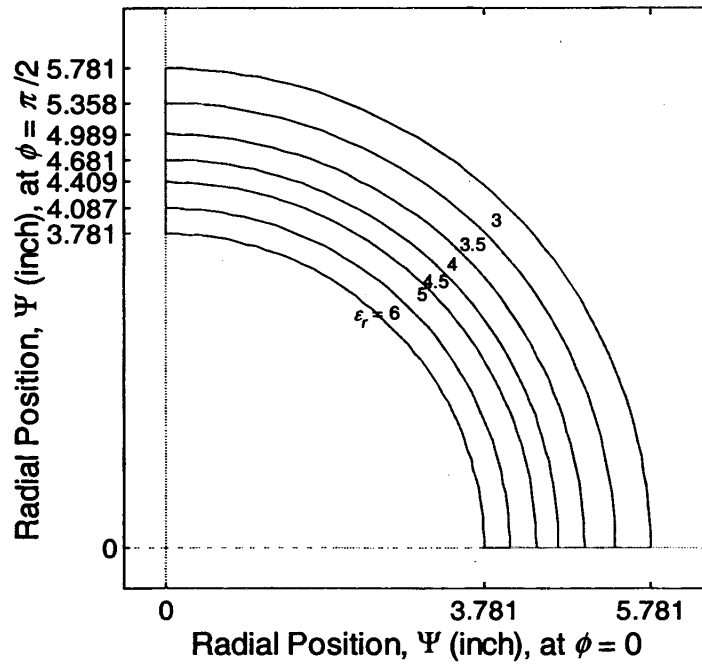
Figure 4. Top view of the layered bend design. Dimensions are inches.
