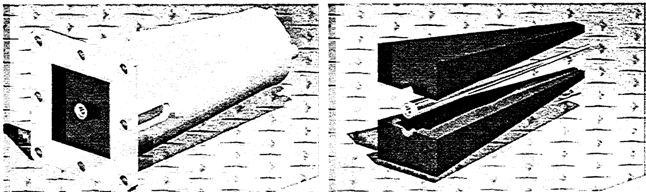
Figure 5. Tapered coaxial transmission line section CAD model. The taper provides a 50 \Omega transition between the square coaxial geometry and an N-type cable connector. The image on the left is an assembled taper; on the right is an exploded view of the dielectric filler and center conductor.
