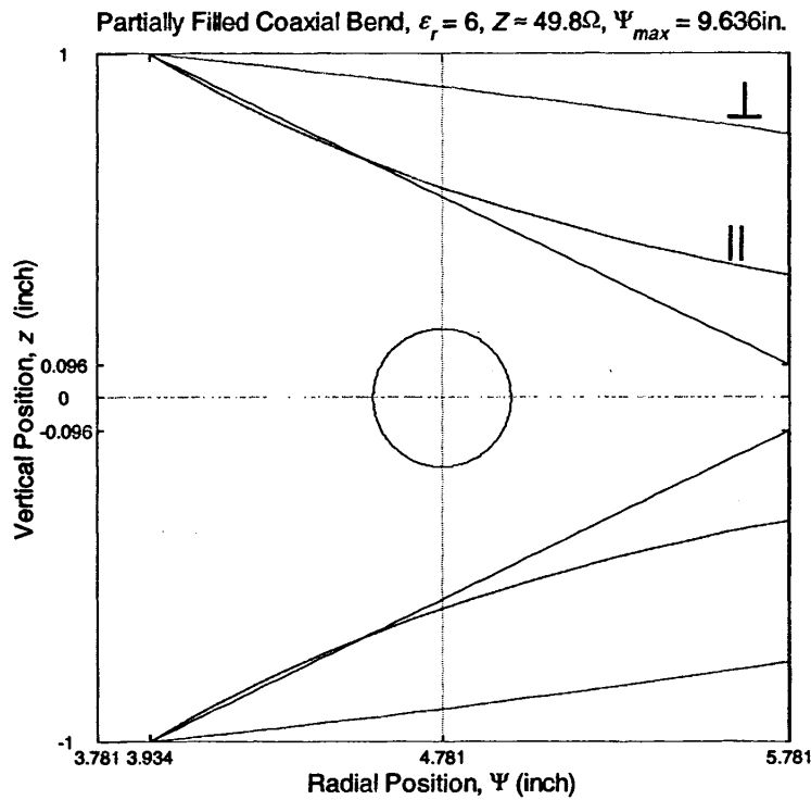
Figure 8. Blunt (top) and sharp (bottom) wedge designs (straight, solid lines). Perpendicular and parallel fill fraction shapes are indicated by the broken line curves. Dimensions are inches.
