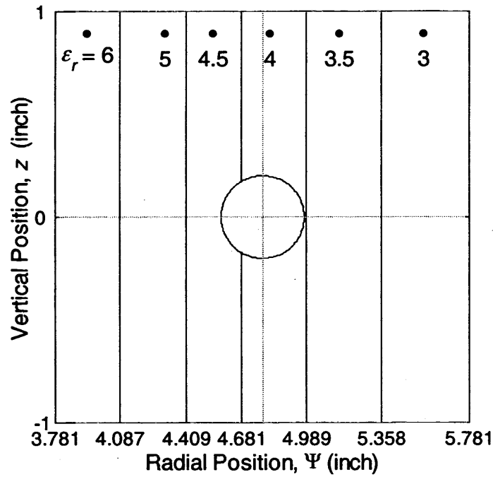
Figure 3. Geometry of the finite element model of the cross section of the layered bend. The center conductor diameter is 1.016 cm (0.4"). Dimensions are inches.
