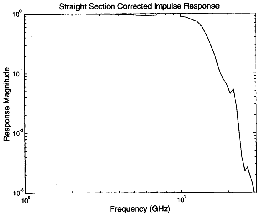
Figure 16. Corrected impulse response for the 19.08 cm (7.51") straight section filled with a uniform \epsilon_r = 4 dielectric. The FWHM of the time-domain peak is 40 ps. A 5 th order modified Butterworth filter with a 15 GHz cutoff was used in deconvolving the system response from the raw data.
