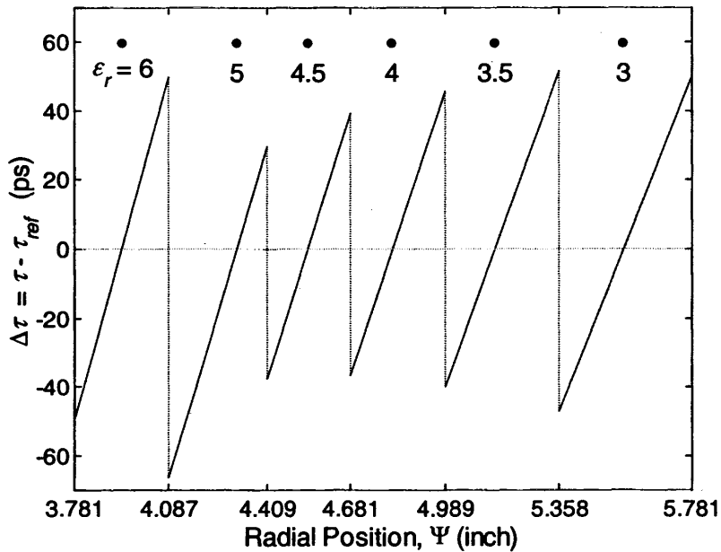
Transit Time Variation for a Layered Coaxial Bend, \Psi_{max} = 9.636\text{in.}
