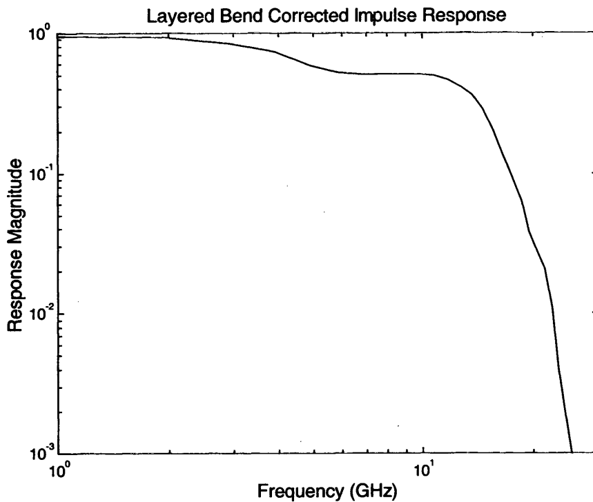
Figure 21. Corrected impulse response for the six-layer laminated bend. The FWHM of the time-domain peak is 44 ps, only 4 ps wider than the corrected response for the comparable straight section of transmission line filled with a uniform dielectric. A 5 th order modified Butterworth filter with a 15 GHz cutoff was used in deconvolving the system response from the raw data.
