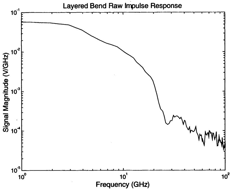
Figure 20. Raw impulse response for the six-layer laminated bend. The FWHM of the time-domain peak is 70 ps, only 15 ps wider than that observed for the comparable straight section of transmission line filled with a uniform dielectric.
