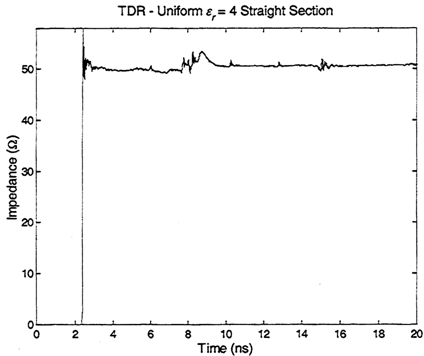
Figure 14. TDR of the straight section filled with a uniform \epsilon_r = 4 dielectric. The small bump at 10.3 ns is the taper-to-straight section interface. The even smaller bump at about 12.8 ns is the interface to the output taper. Within the straight section, the impedance is 50.5 \Omega .
