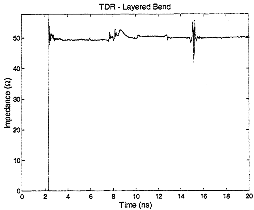
Figure 19. TDR of the six-layer dielectric laminate-filled bend. The small bump at 10.1 ns is the taper-to-bend interface. The other small bump at about 12.8 ns is the interface to the output taper. Within the bend, the impedance is a flat 50.4 \Omega .
