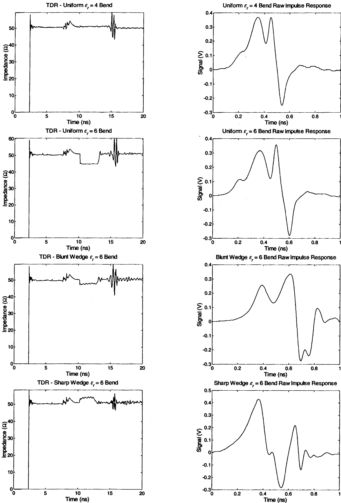
Figure 17. TDR and impulse response data for uniform and partially filled bends. Note the enhanced ringing at the output N/SMA adapter, and, for the wedges, within the bend itself. None of these bends is able to transmit a reasonable facsimile of an impulse.
