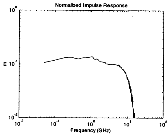
Figure 2.5. Normalized impulse response.
