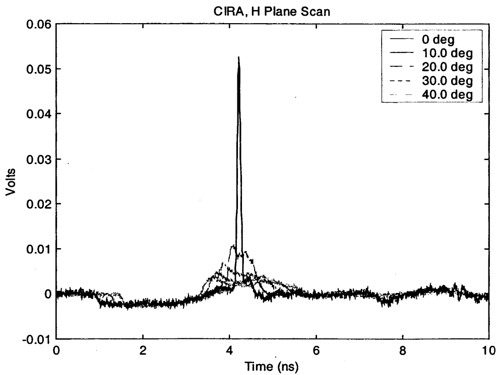
Figure 4.13 Raw voltage at several angles in H plane.
