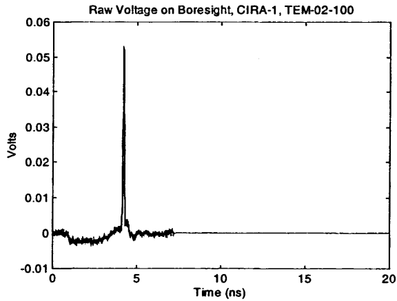
Figure 4.2 Raw data on boresight with ground bounce removed and zero-padded.
