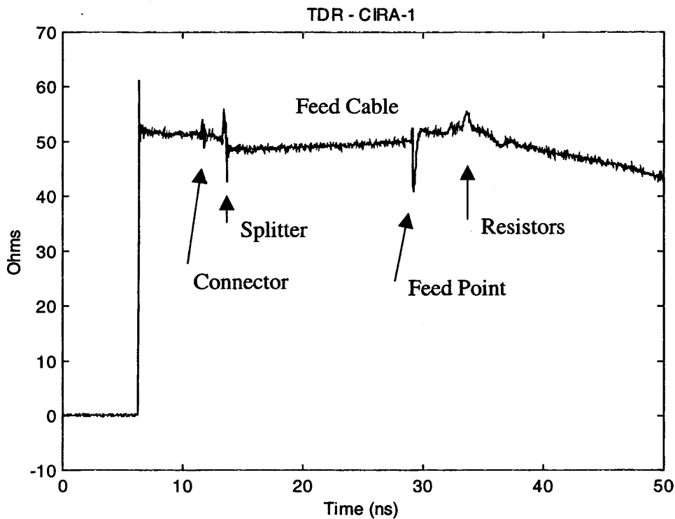
Figure 4.1 TDR of CIRA.
