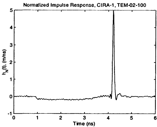
Figure 4.3 Expanded normalized impulse response [2] (FWHM = 73 ps, left, 68 ps, right).
