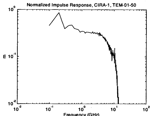
Figure 4.4 Normalized impulse response of the CIRA on boresight.
