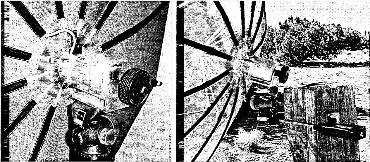
Figure 3.2 Back side of CIRA mounted on tripod (left) and clamp (right).
