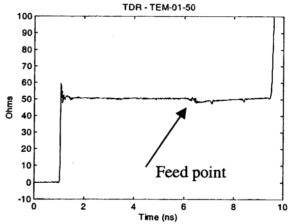
Figure 2.8. TDR of the FRI-TEM-01-50.
