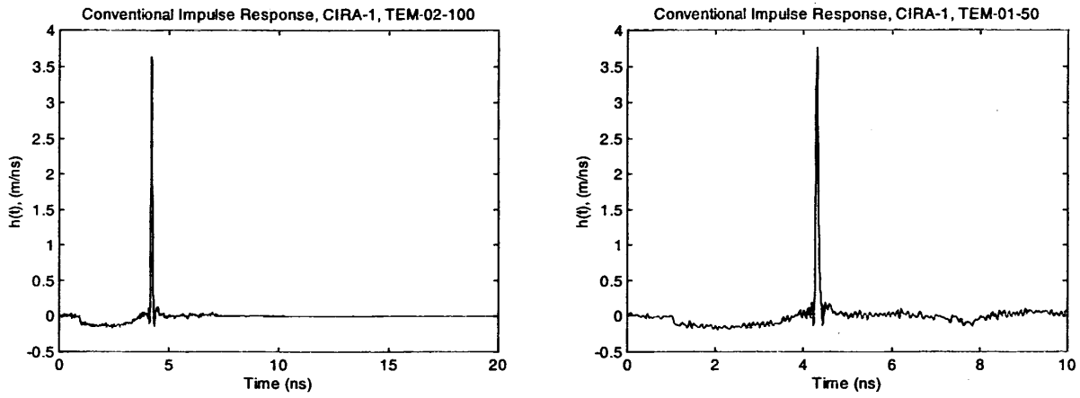
Figure 4.6 Conventional impulse response, h(t) [2]
