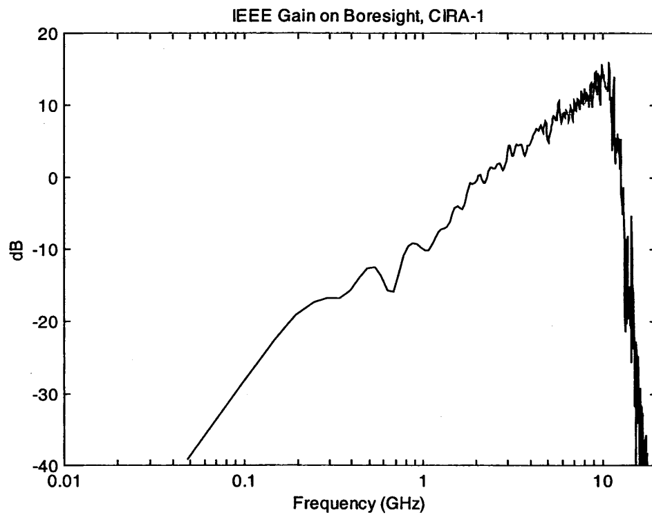
Figure 4.9 IEEE gain of cross polarization response.
