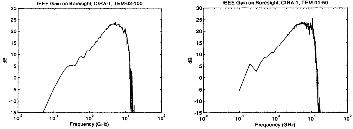
Figure 4.5 IEEE gain of the CIRA on boresight.
