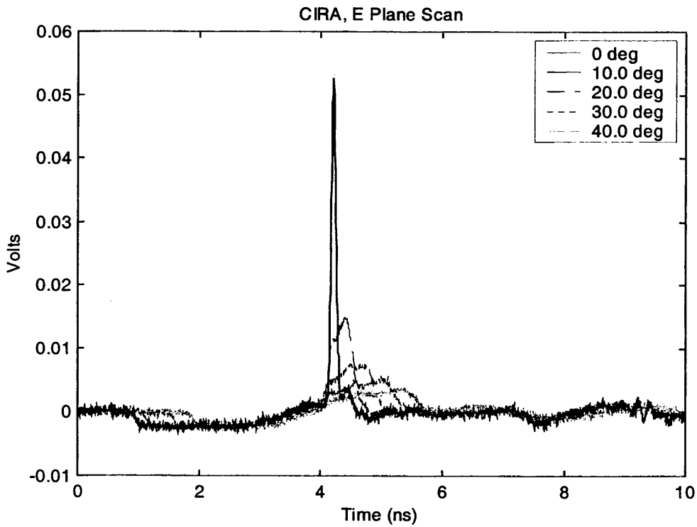
Figure 4.15 Raw voltage measurements at several angles in E plane.
