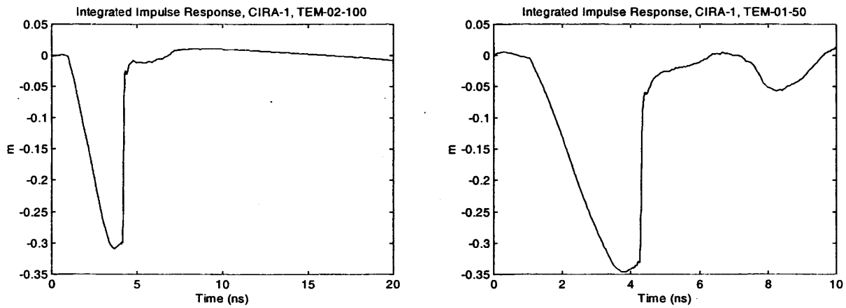
Figure 4.7 Integrated impulse response ( h_a = 0.30 m)
