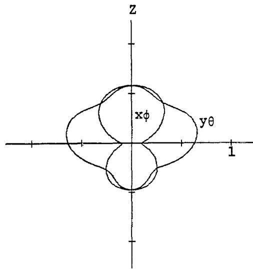
(b) two mode currents
