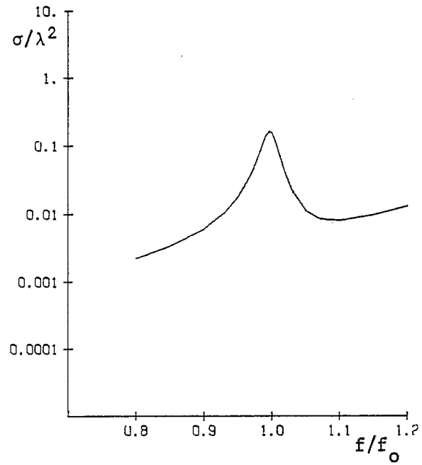
(b) two mode voltages
