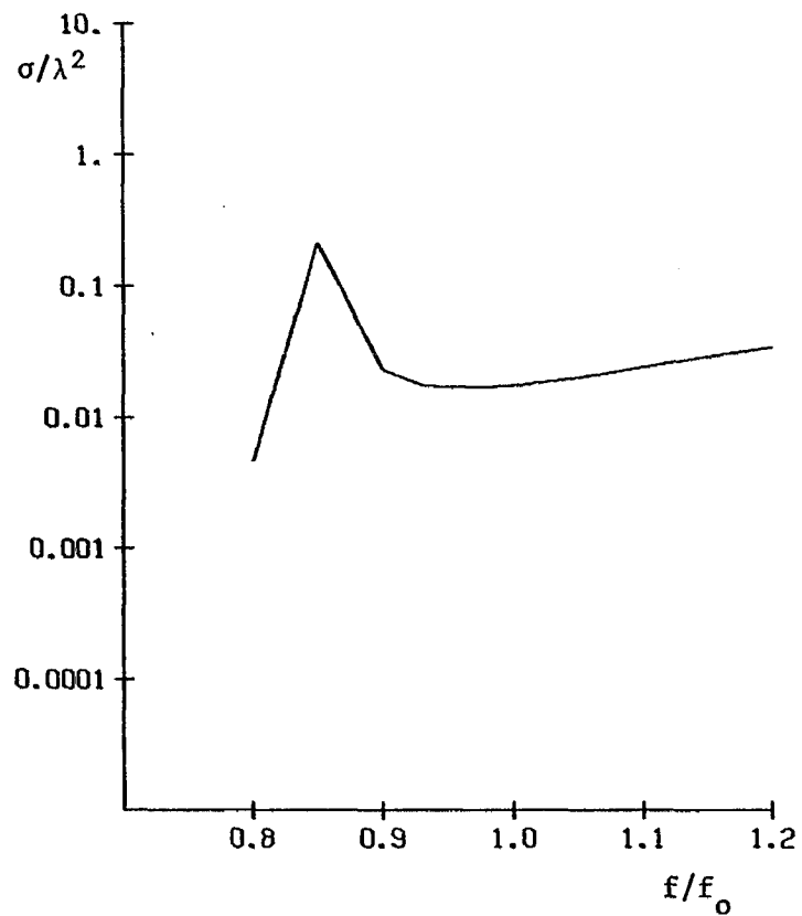
(a) open-circuited scatterer
