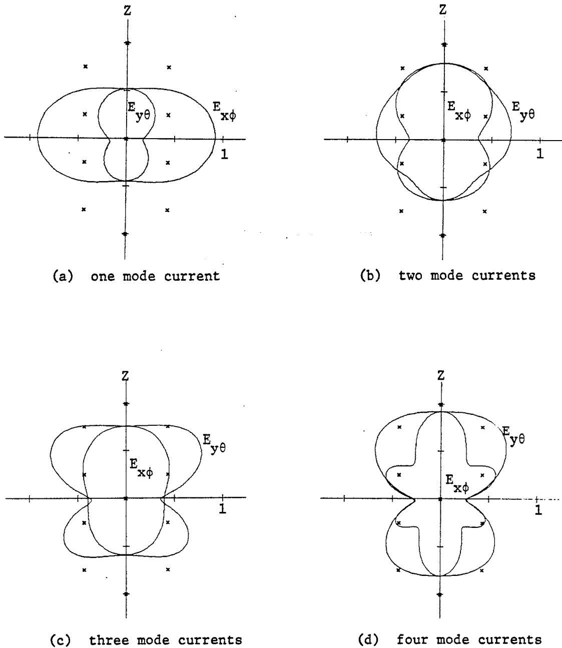
Fig. 5. Field magnitude pattern synthesis using real mode currents as a basis. Crosses denote the desired pattern. Curves labeled E_{x\phi} denote |E_\phi| in the x=0 plane. Curves labeled E_{y\theta} denote |E_\theta| in the y=0 plane.
