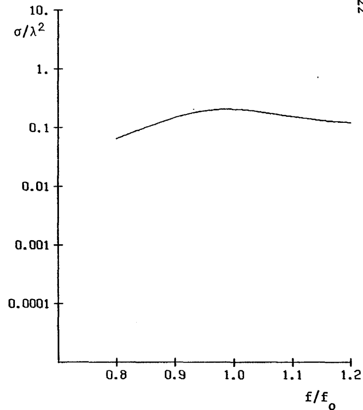
(b) short-circuited scatterer
