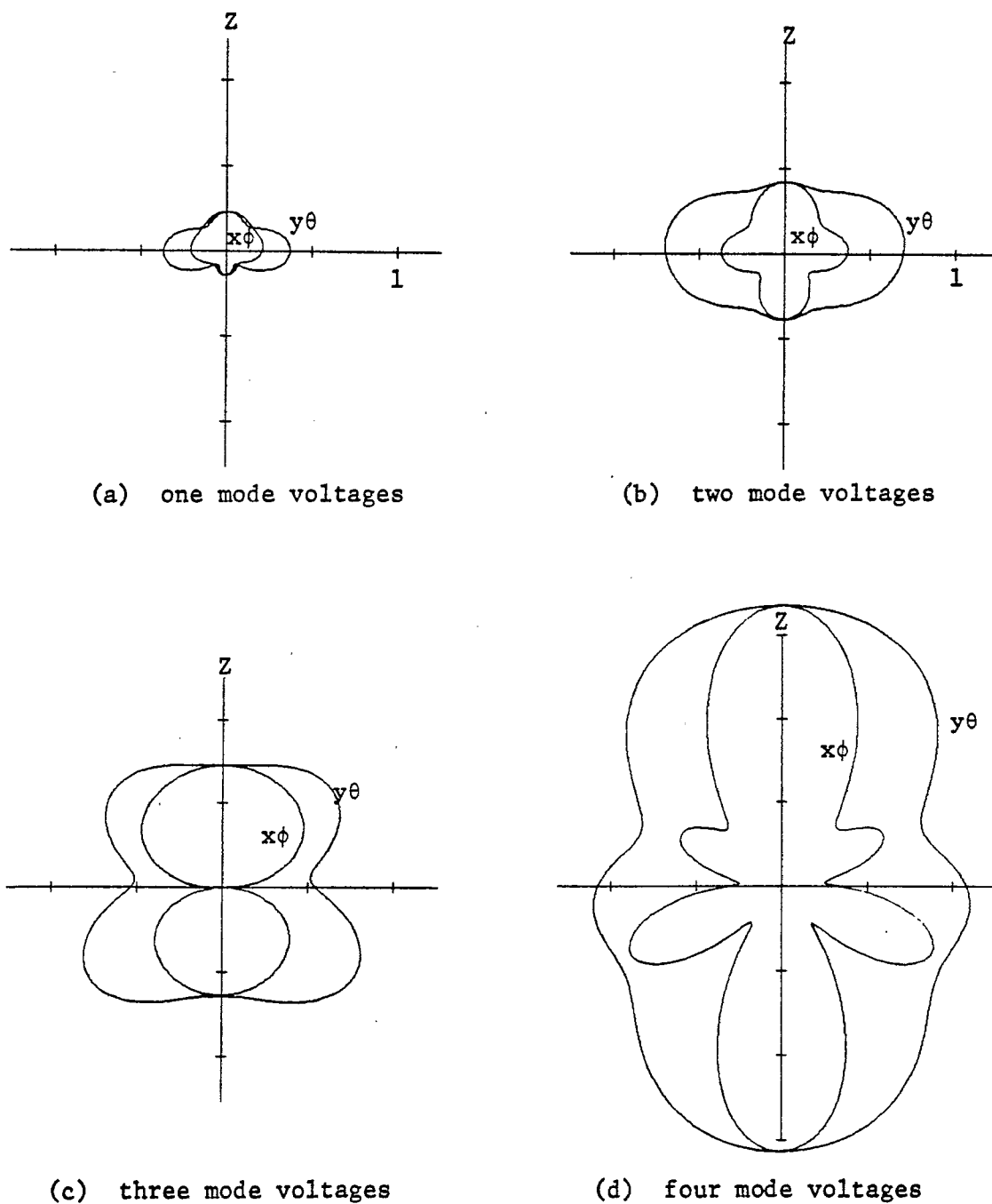
Fig. 17. Bistatic scattering patterns ( \sqrt{\sigma}/\lambda ) for the wire object of Fig. 1 loaded to resonate the port voltages which synthesize the patterns of Fig. 16. Curves labeled x\phi denote \phi polarization in the x=0 plane. Curves labeled y\theta denote \theta polarization in the y=0 plane.
