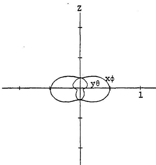
(a) one mode current
