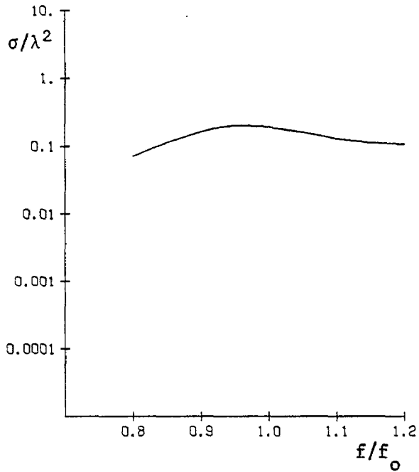
(a) one mode current
