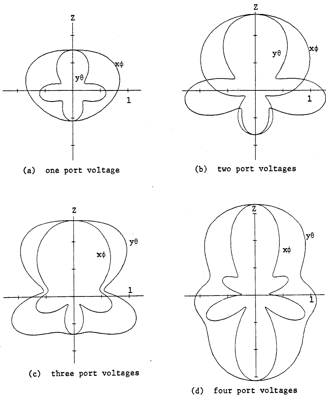
Fig. 14. Bistatic scattering patterns ( \sqrt{\sigma}/\lambda ) for the wire object of Fig. 1 loaded to resonate the port voltages which synthesize the patterns of Fig. 13. Curves labeled x\phi denote \phi polarization in the x=0 plane. Curves labeled y\theta denote \theta polarization in the y=0 plane.
