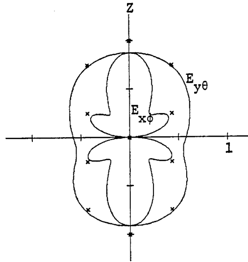
(b) four mode currents, compare with Fig. 5d.
