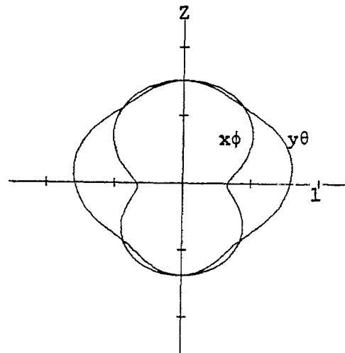
(b) two mode currents
