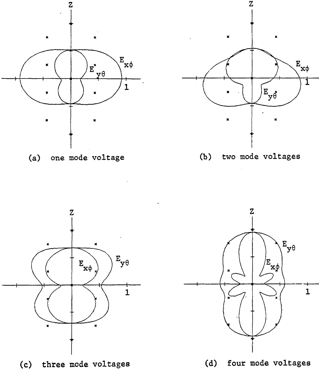
Fig. 16. Field magnitude pattern synthesis using real mode voltages as a basis. Crosses denote the desired pattern. Curves labeled E_{x\phi} denote |E_\phi| in the x=0 plane. Curves labeled E_{y\theta} denote |E_\theta| in the y=0 plane.
