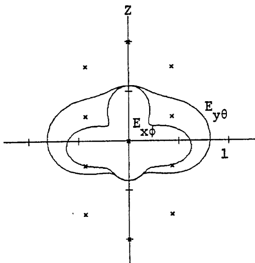
(c) two mode voltages, compare with Fig. 16b.
