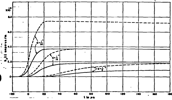
Fig. 9. Aluminum spherical shell. t_1 = 6 \mu s .
