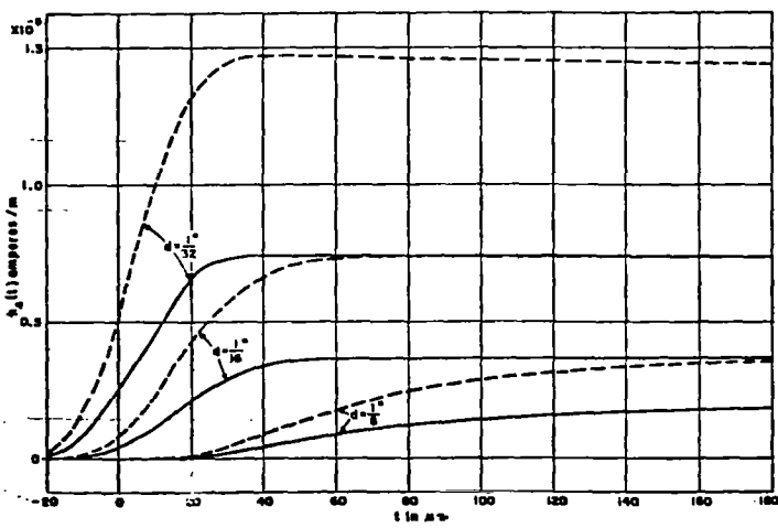
Fig. 10. Aluminum spherical shell. t_1 = 12 \mu s .
