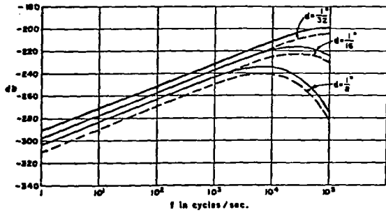
Fig. 2. Aluminum spherical shell. Steady-state transfer characteristic relating E_a(f) to E_0(f) .
