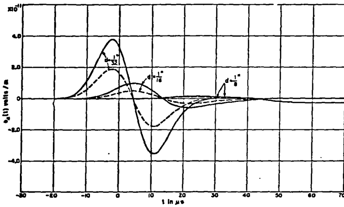
Fig. 3. Aluminum spherical shell. t_1 = 6 \mu s .
