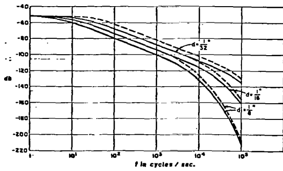
Fig. 8. Aluminum spherical shell. Steady-state transfer characteristic relating H_c(f) to E_o(f) .
