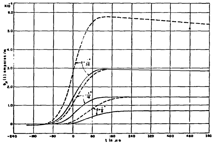
Fig. 12. Aluminum spherical shell. t_1 = 48 \mu s .
