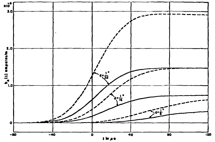
Fig. 11. Aluminum spherical shell. t_1 = 24 \mu s .
