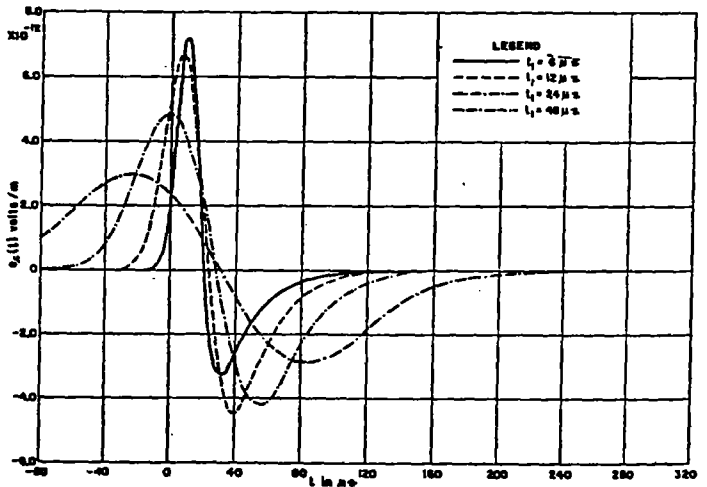
Fig. 7. Copper spherical shell (shielded room).
