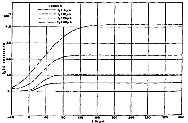
Fig. 13. Cooper spherical shell (shielded room).
