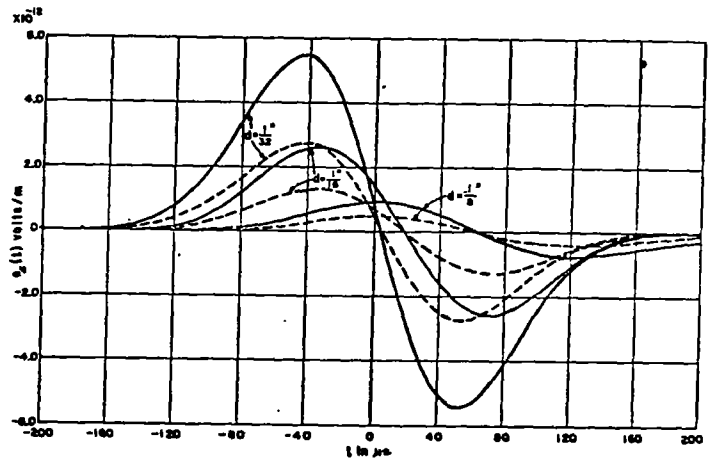
Fig. 6. Aluminum spherical shell. t_1 = 48 \mu s .
