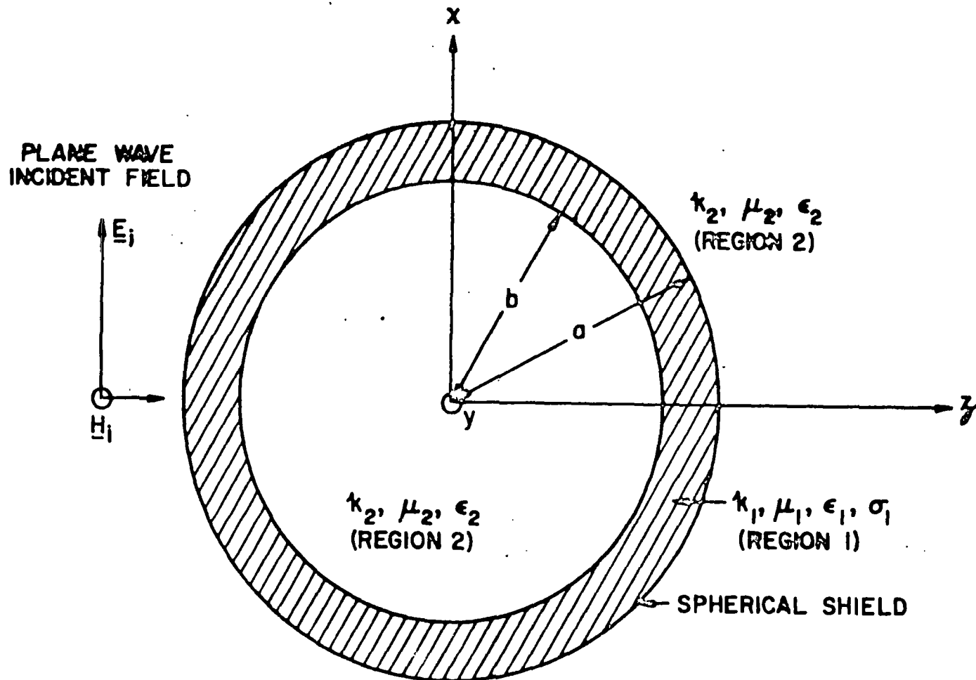
FIGURE 1: SPHERICAL SHIELD. THE FIELDS \underline{E}_i AND \underline{H}_i ARE POLARIZED PARALLEL TO THE x AND y AXES, RESPECTIVELY.
