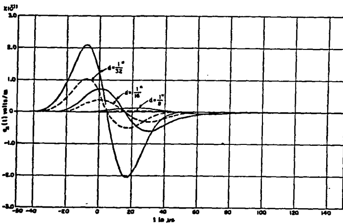
Fig. 4. Aluminum spherical shell. t_1 = 12 \mu s .
