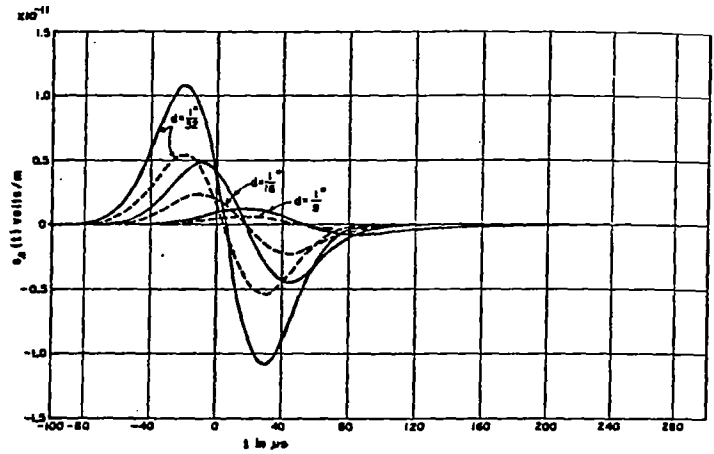
Fig. 5. Aluminum spherical shell. t_1 = 24 \mu s .
